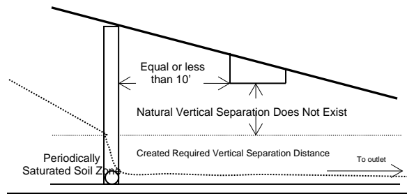
Figure 1. Drainage Method – Upslope French Drain
