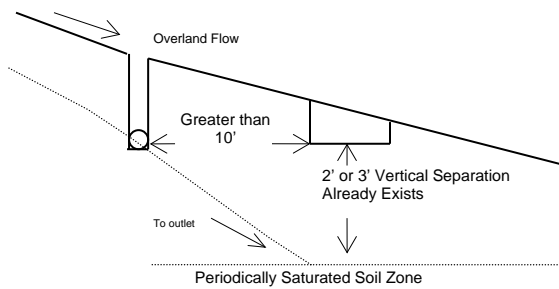
Figure 3. Diversion Method – Interceptor Drain
