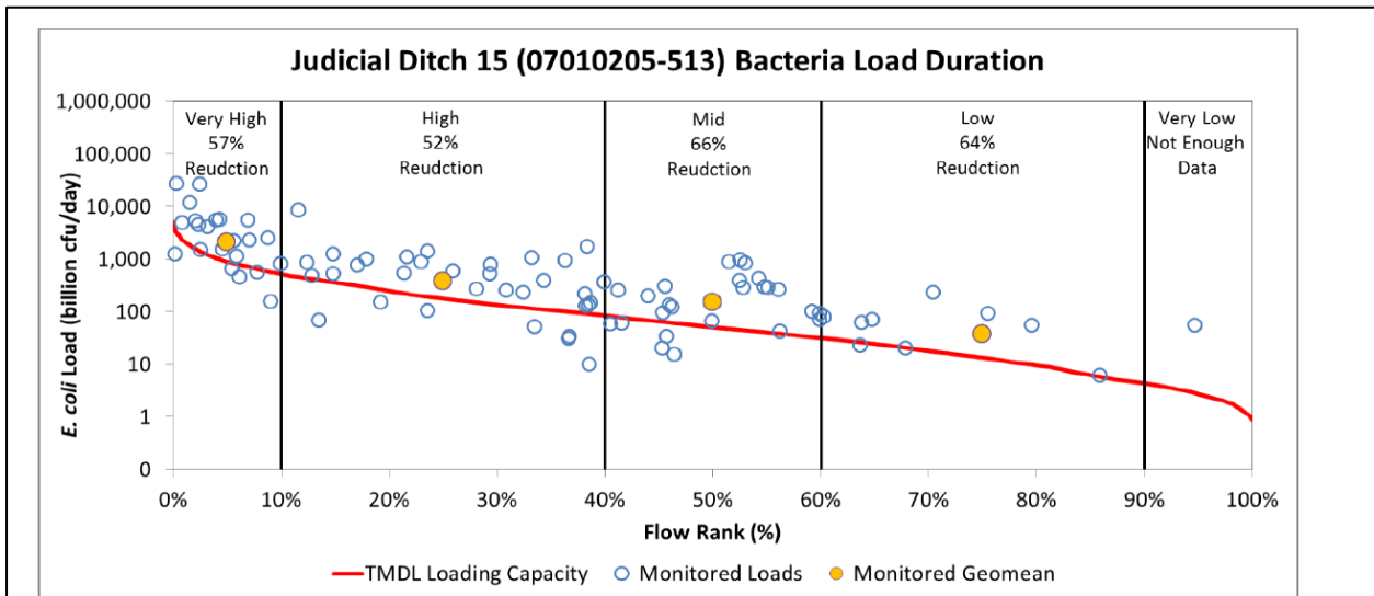
Figure 4-6. E. coli monitored loads, load standard and load reductions for JD15 reach 513.
