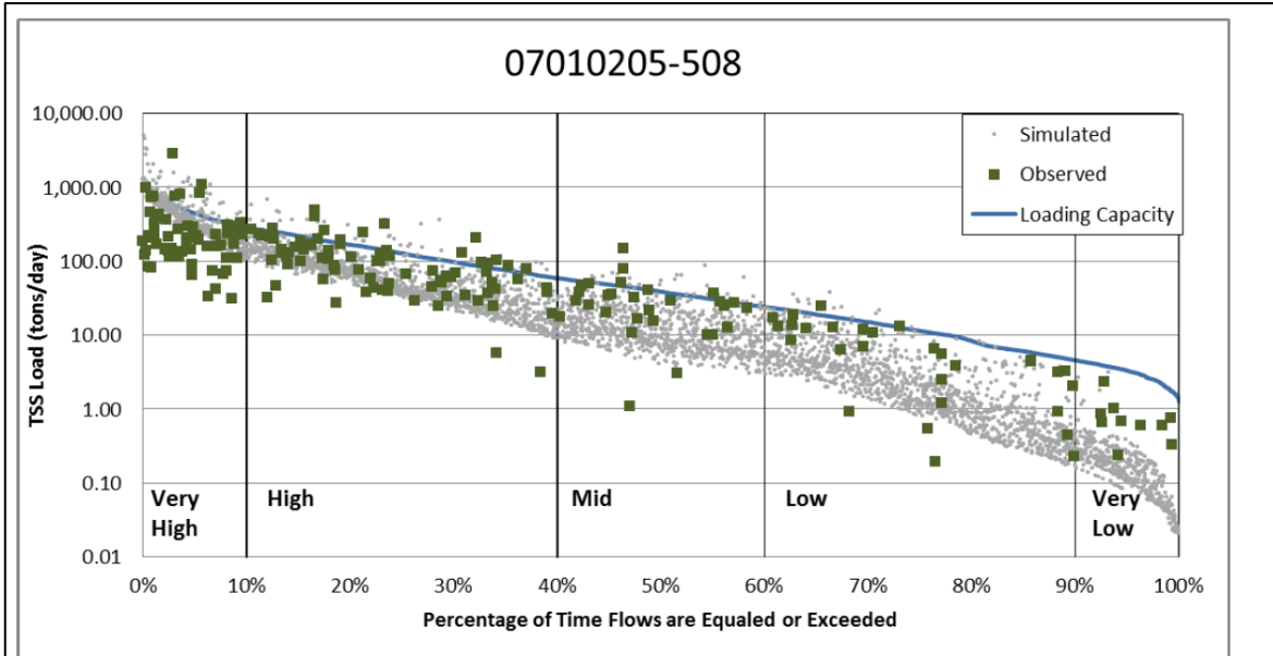
Figure 4-5. South Fork Crow (07010205-508) TSS load duration curve.
