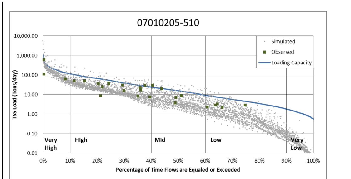
Figure 4-3. South Fork Crow (07010205-510) TSS load duration curve.
