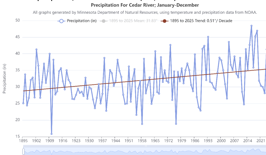
Figure 4. Annual precipitation, Cedar River Watershed (DNR, 2025b).
