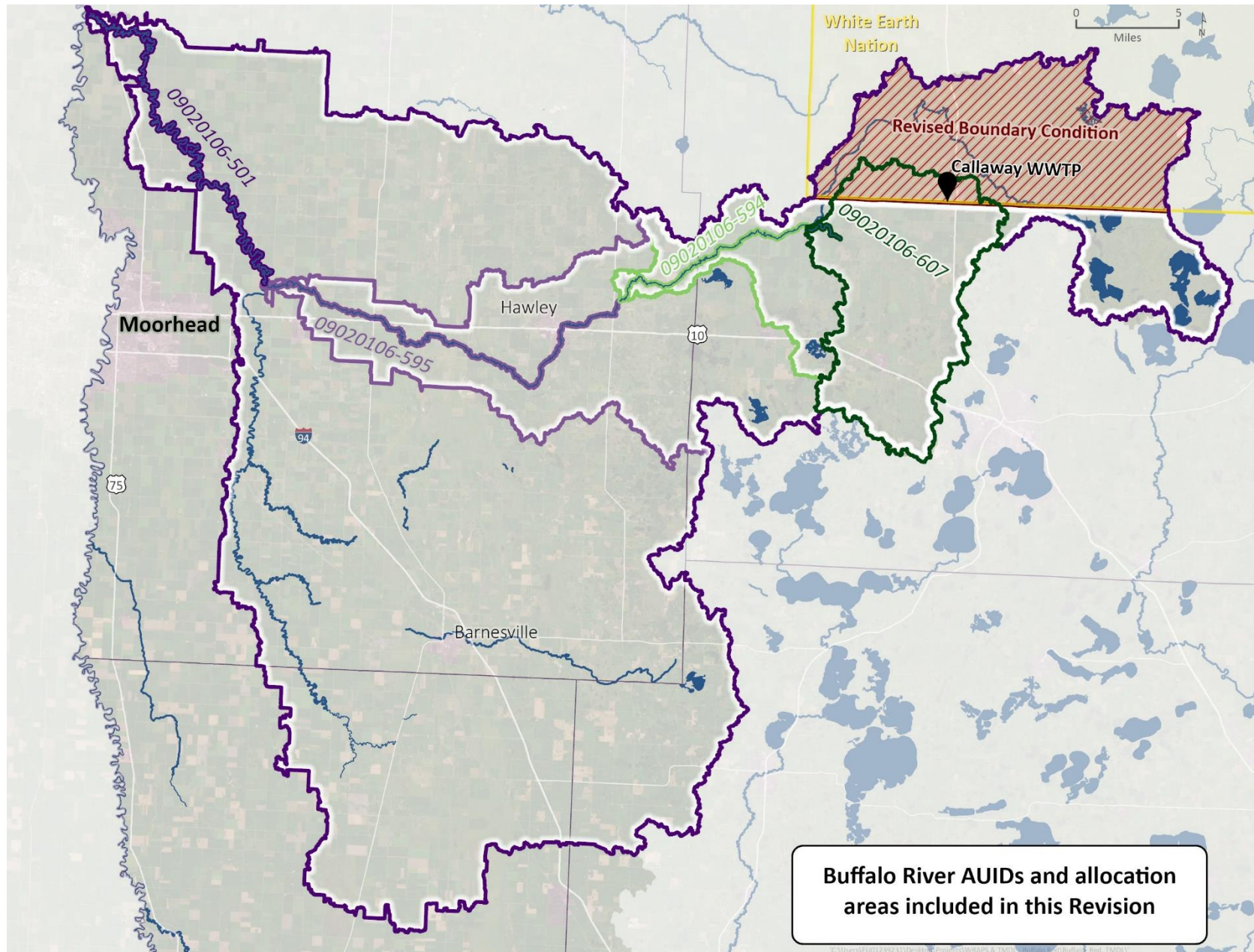
Figure 1. Boundary condition areas added for the Buffalo River and Becker County Ditch 15 as part of the revisions of the 2017 approved Buffalo River Watershed TMDL.
