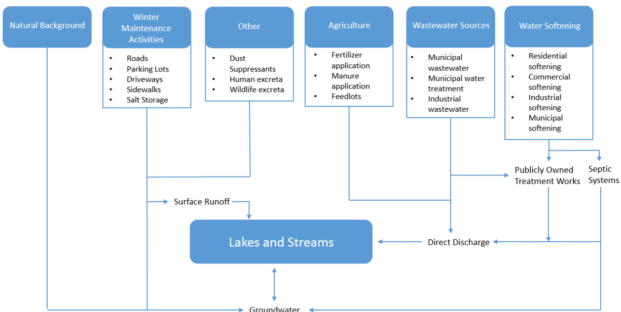
Figure 27. Conceptual model of anthropogenic sources of chloride and pathways
