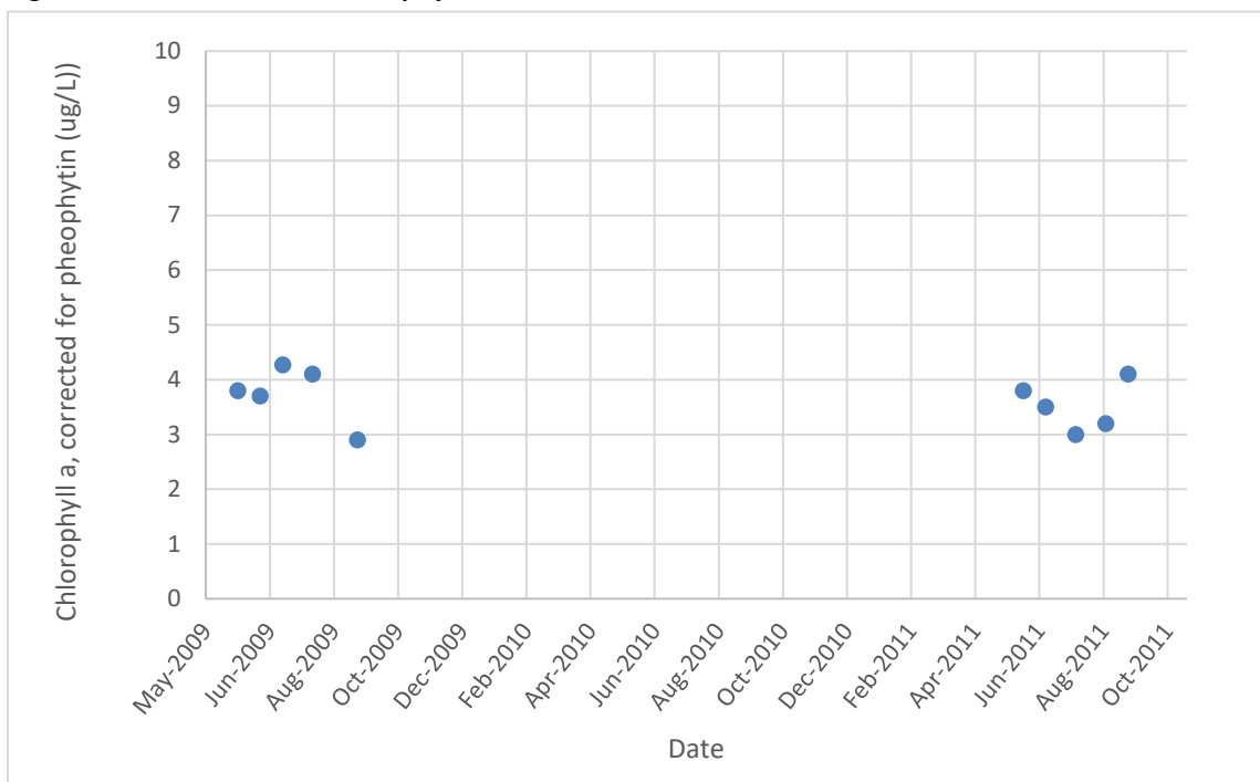
Figure 5. Steamboat Lake chlorophyll-a concentrations
