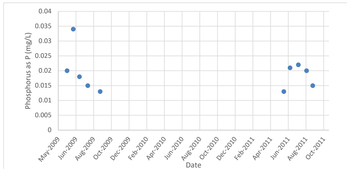
Figure 2. Steamboat Lake phosphorus concentrations
