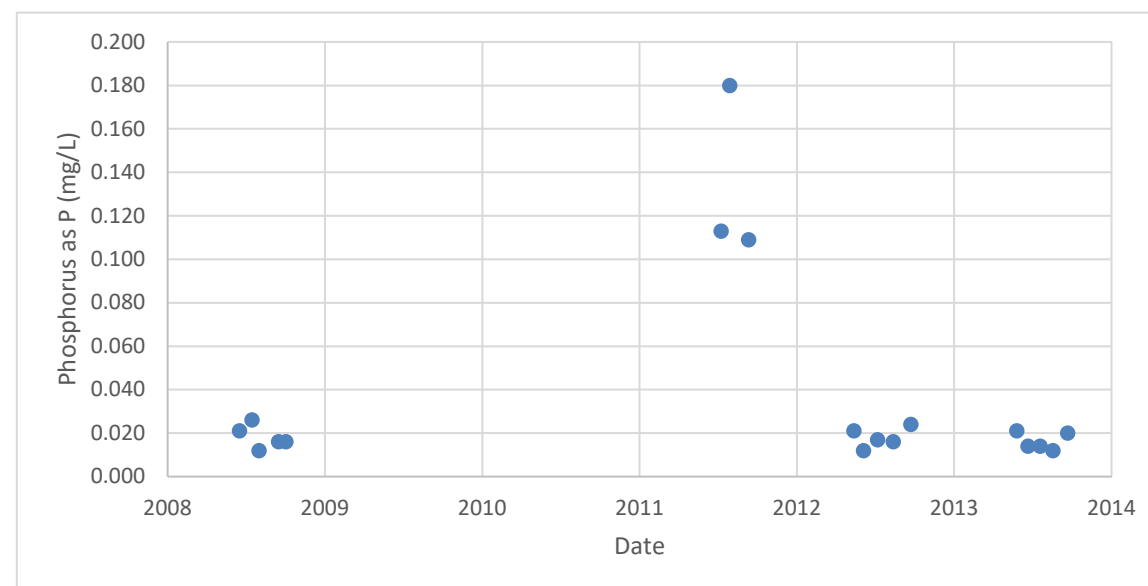
Figure 3. Portage Lake phosphorus concentrations
