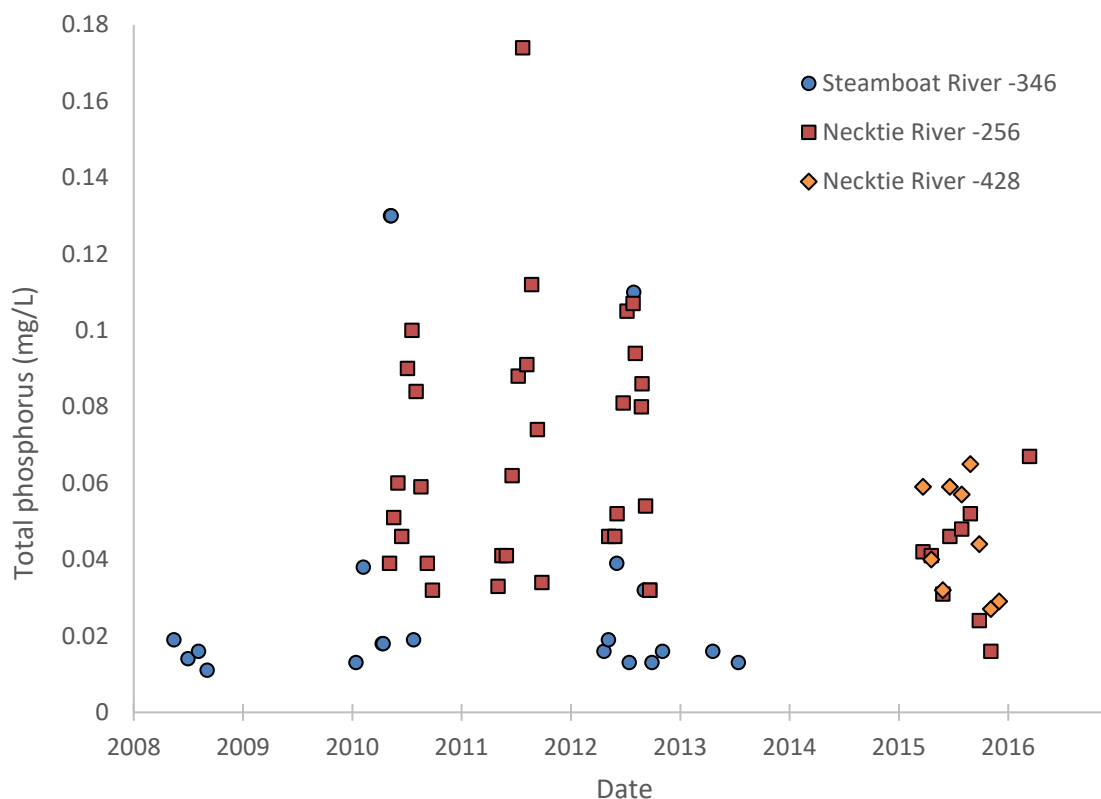
Figure 12. Total phosphorus data for the Steamboat and Necktie River monitoring sites
