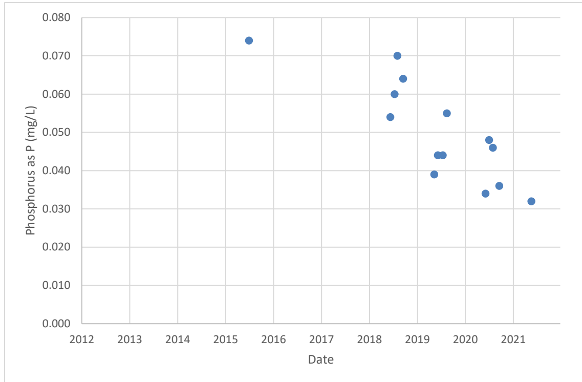
Figure 4. Hart Lake phosphorus concentrations
