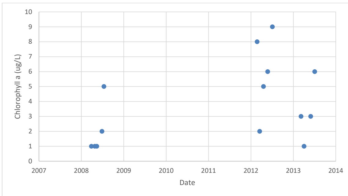
Figure 6. Portage Lake chlorophyll-a concentrations
