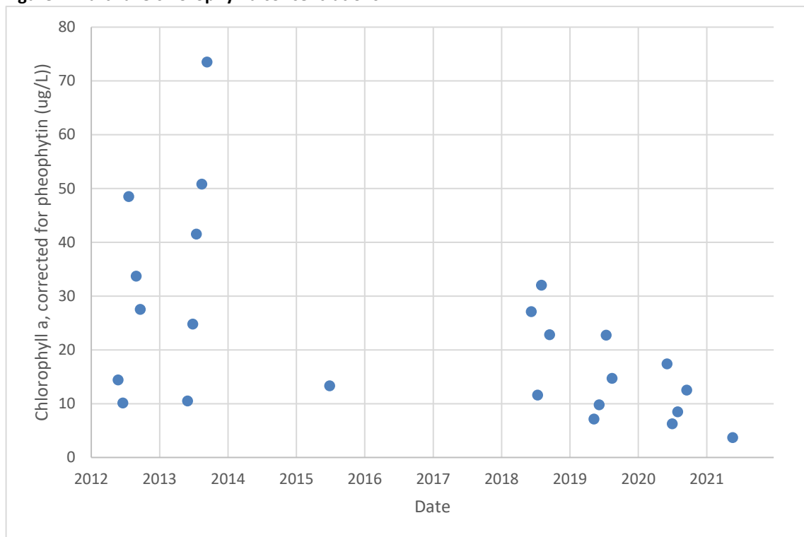
Figure 7. Hart Lake chlorophyll-a concentrations
