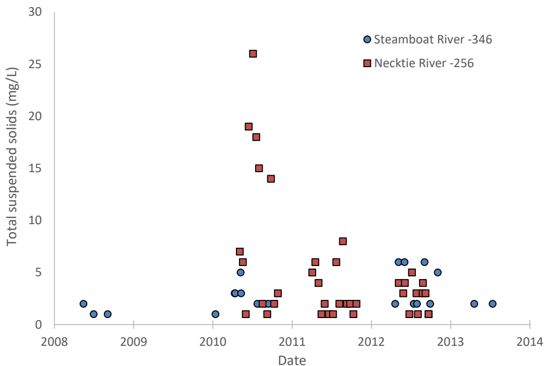
Figure 11. Total suspended solids data for the Steamboat and Necktie River monitoring sites
