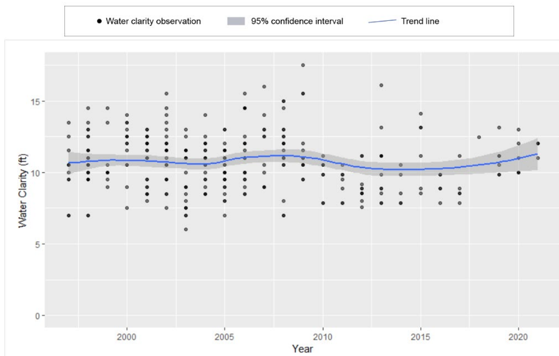
Figure 8. Water clarity and trend analysis for Portage Lake (MPCA 2023)
