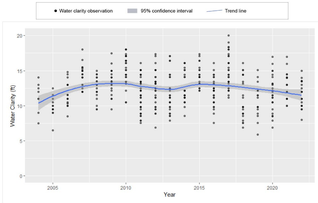
Figure 9. Water clarity and trend analysis for Steamboat Lake (MPCA 2023)
