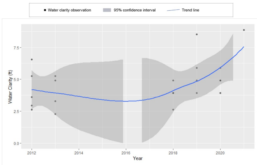
Figure 10. Water clarity and trend analysis for Hart Lake (MPCA 2023)
