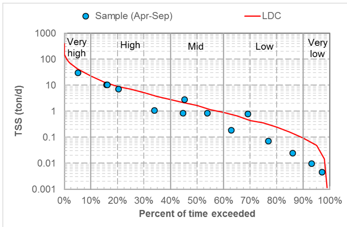
Figure 12. TSS load duration curve, Rice Creek
