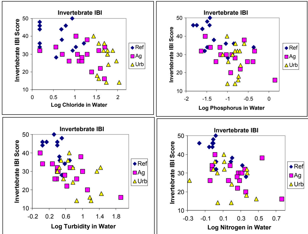
Figure 7. Invertebrate Index of Biological Integrity (IBI) scores plotted against chloride, phosphorus and nitrogen in the water (log of concentration in mg/L) and turbidity (in ntu).
