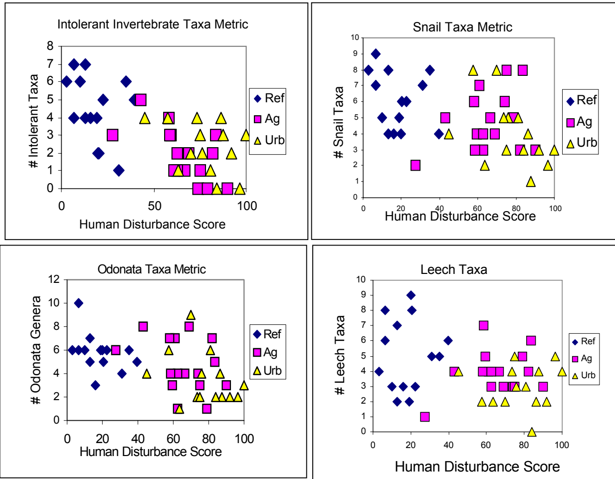
Figure 3. Invertebrate metrics plotted against the human disturbance gradient scores for 44 large depressive wetlands in Minnesota: Intolerant Taxa, Snail Taxa, Odonata Taxa and Leech Taxa metrics.
