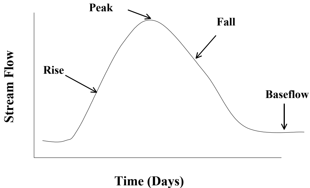
Figure 4. A Storm Hydrograph
