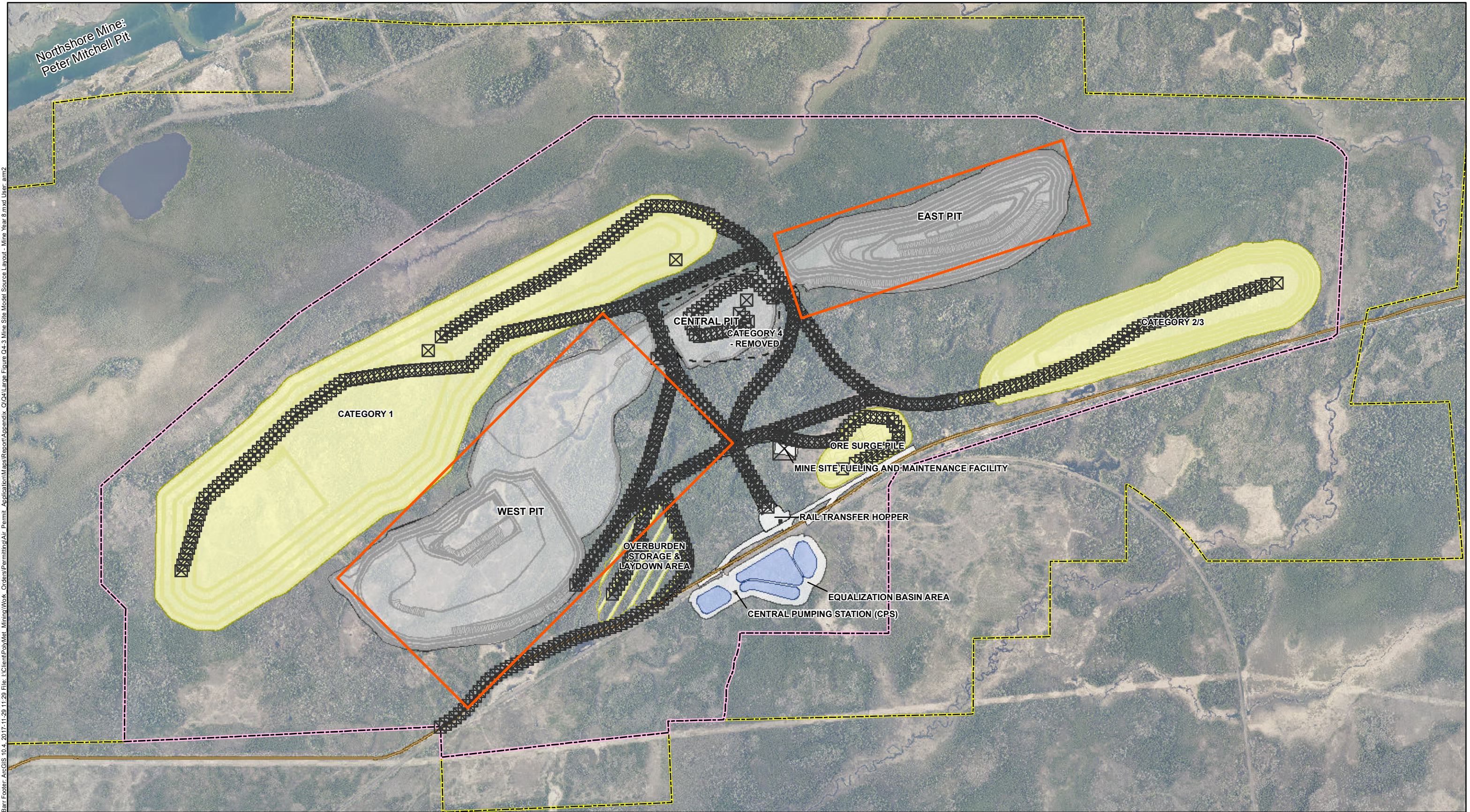
MINE SITE MODEL SOURCE LAYOUT - MINE YEAR 8 NorthMet Project Poly Met Mining, Inc. Large Figure Q4-3 Appendix Q-4 Total Facility Modeling
