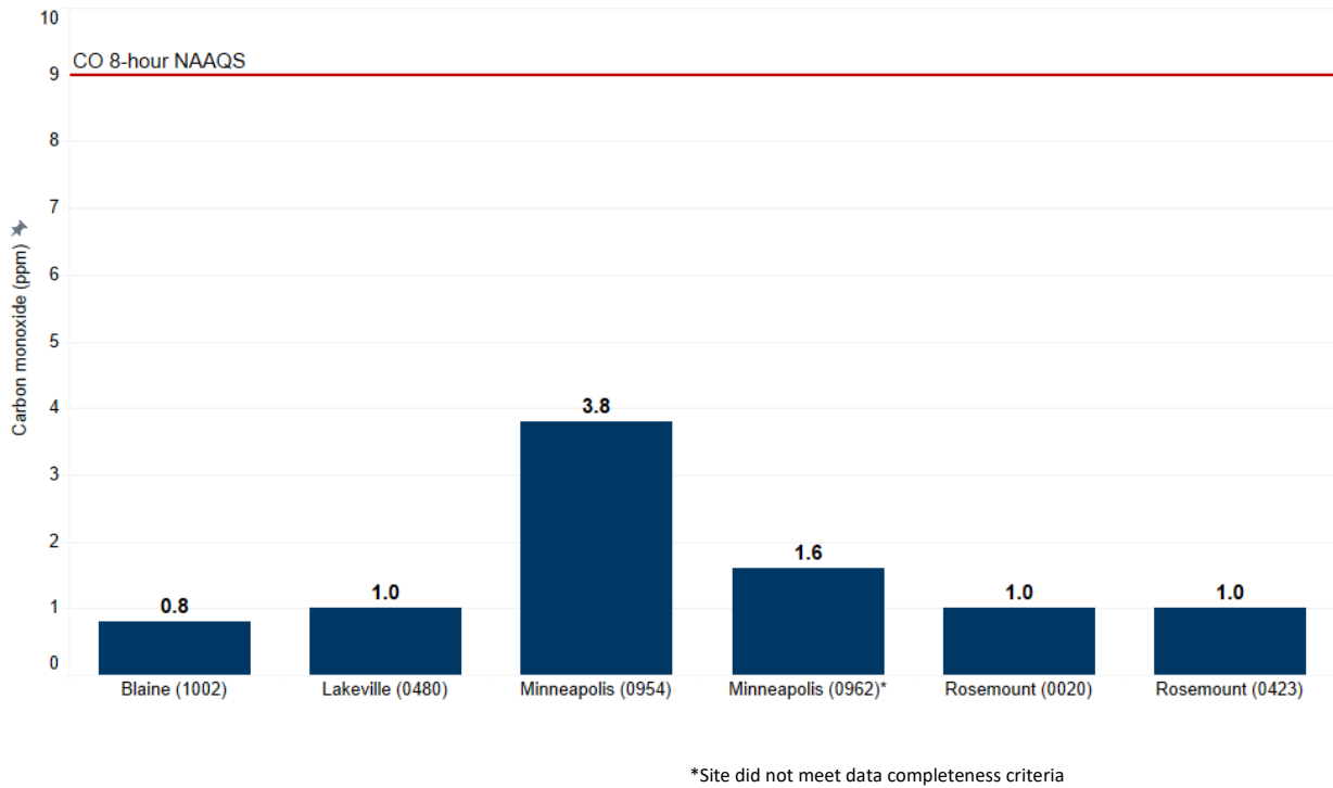
Figure 32. 2023 design values for CO compared to the 8-hour NAAQS.
