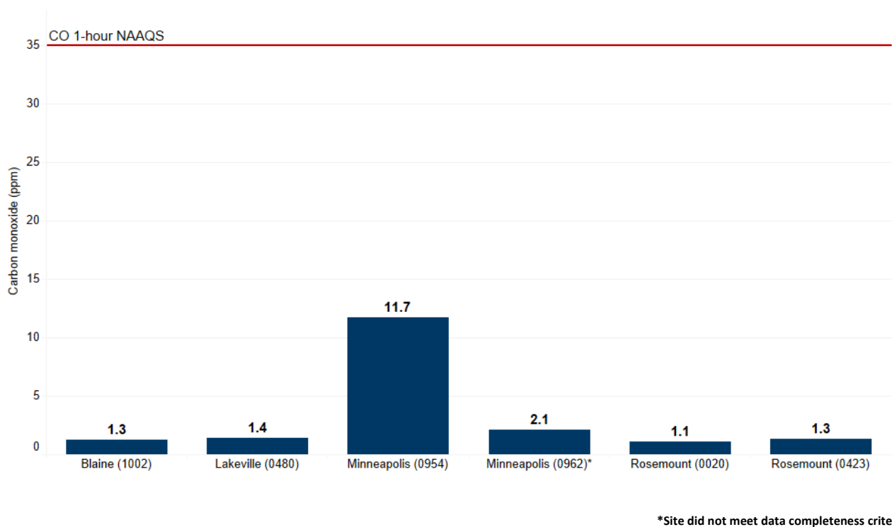
Figure 33. 2023 CO design values compared to the 1-hour average NAAQS.
