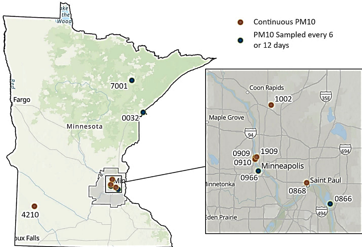
Figure 19. 2024 PM 10 monitoring sites in Minnesota.
