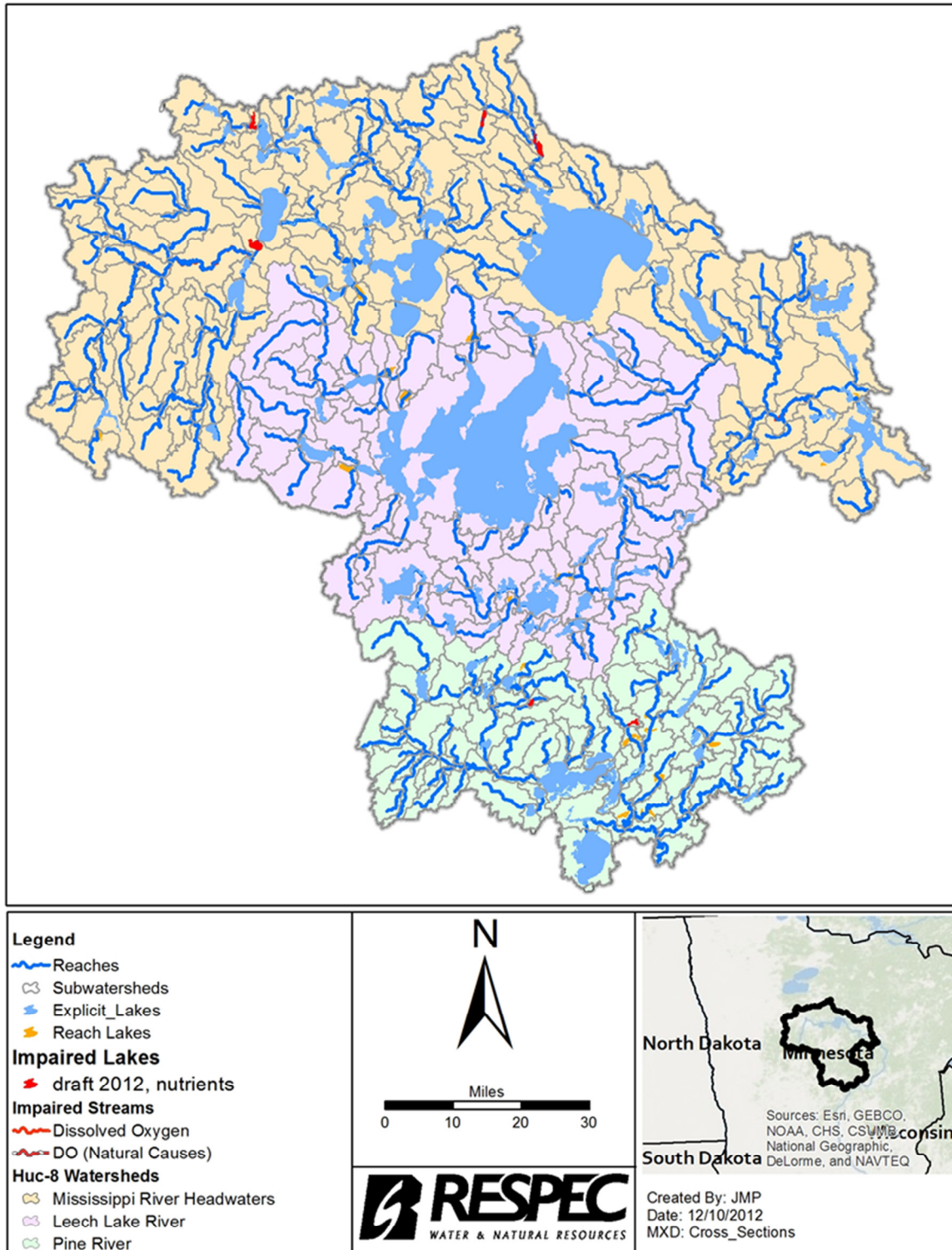
Figure 5. Mississippi River Headwaters, Leech Lake River, and Pine River Watersheds Subwatershed Boundaries.
