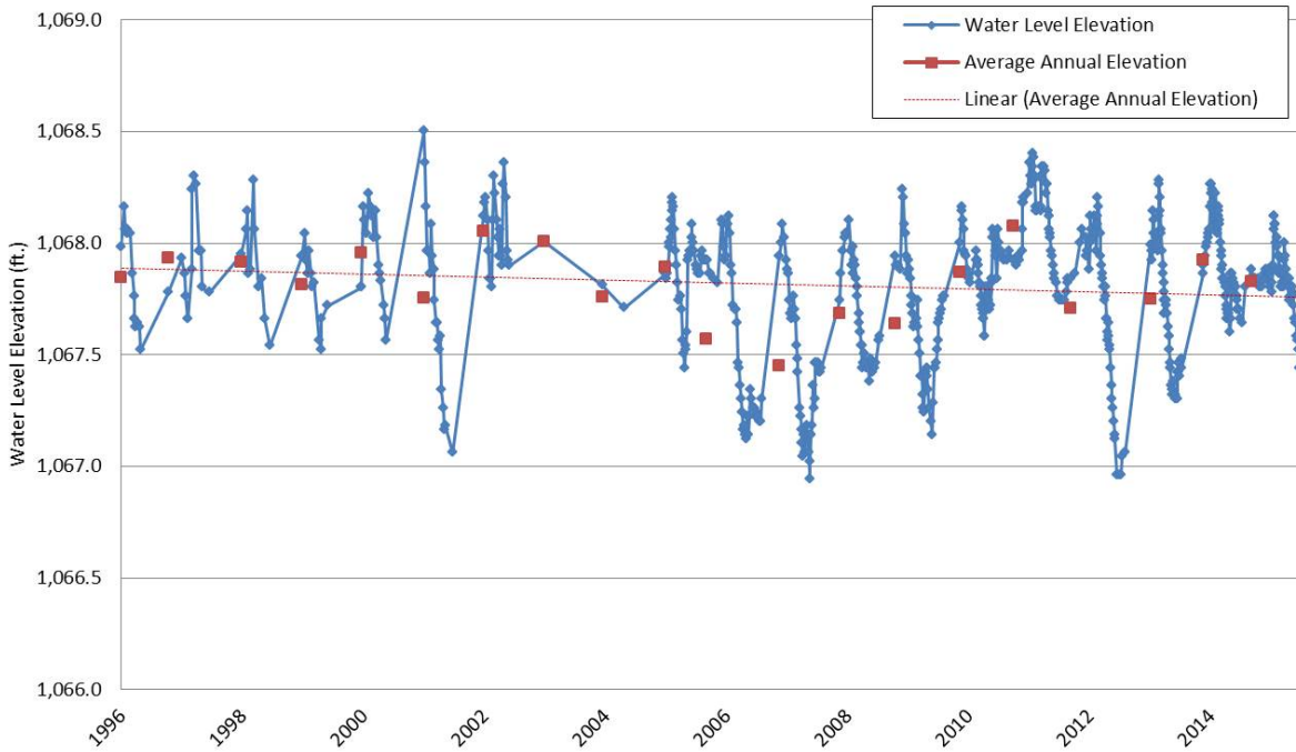
Figure 16: Lake Washington water level elevations (1996-2015)
