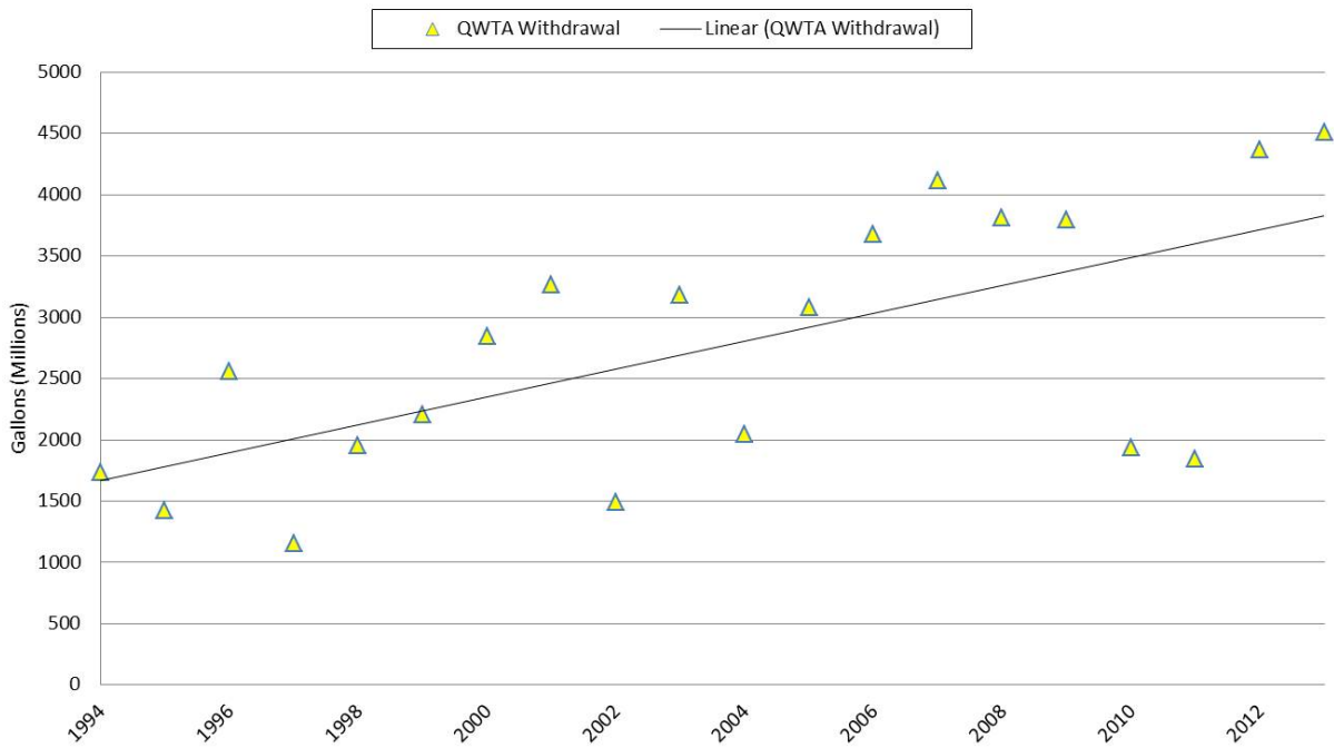
Figure 40: Total annual quaternary water table withdrawals in the North Fork Crow River Watershed (1994-2013)
