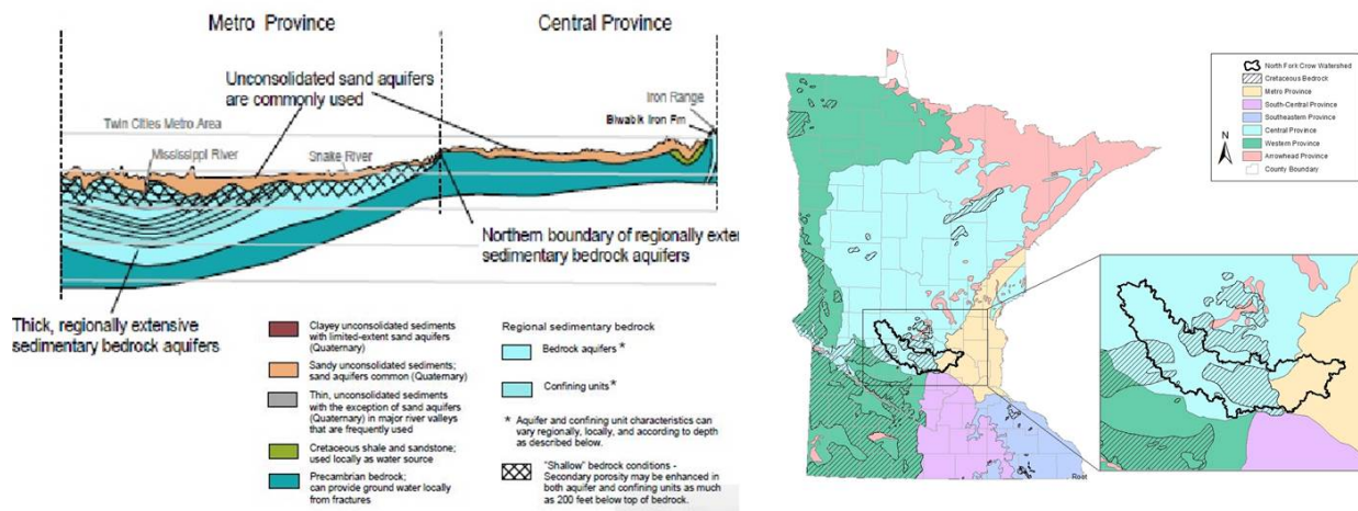
Figure 24: Metro and Central Province generalized cross section (Source: MDNR, 2001)
