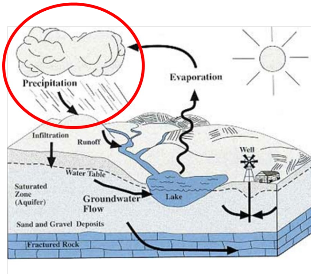
Figure 7: Precipitation within the hydrologic cycle
