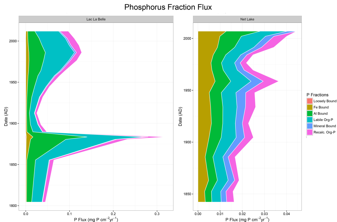
Figure 6b. Flux or accumulation of sediment phosphorus fractions in Lac La Belle and Net Lake cores including Loosely Bound P, Fe-Bound P, Al-Bound P, Labile Organic P, Mineral-Bound P, and Recalcitrant Organic P. The sum of these fractional fluxes equals sediment total phosphorus flux. P fraction flux data shown as accumulation rate (mg P/cm 2 yr) of each P fraction by core date.
