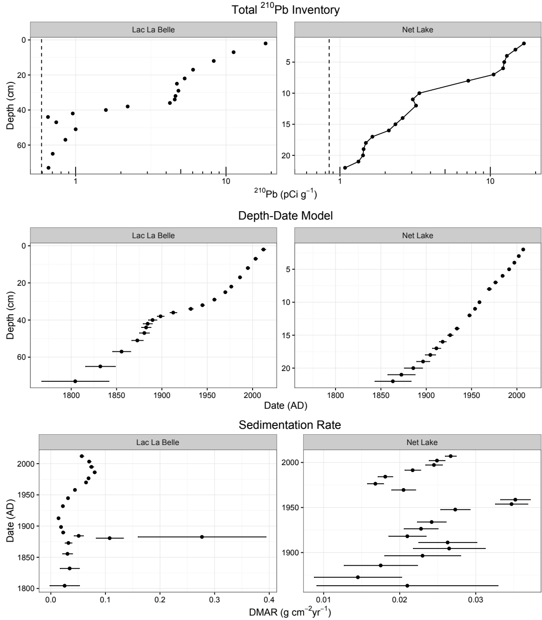
Figure 3. Inventory of 210 Pb by depth (cm), date-depth (cm) model, and bulk sedimentation rates (dry mass accumulation rates, DMAR, g/cm 2 yr) by date (AD) for Net Lake and Lac La Belle. Dashed line in 210 Pb inventory is supported level of 210 Pb. Horizontal bars represent standard error estimates.
