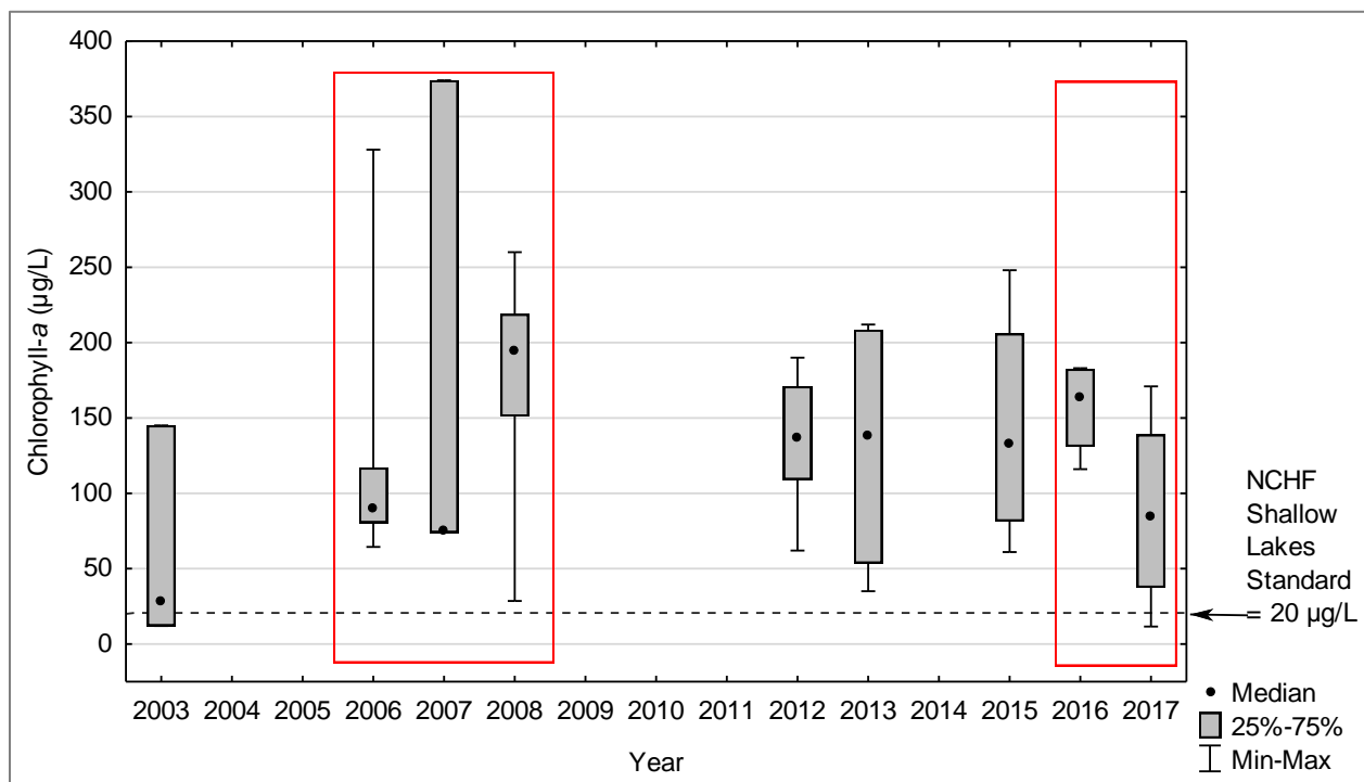
Figure 17. Little Rock Lake chlorophyll- a surface concentrations (June–September); site 05-0013-00-204. Pre-implementation (2006–2008) and post-implementation (2016–2017) periods are highlighted.
