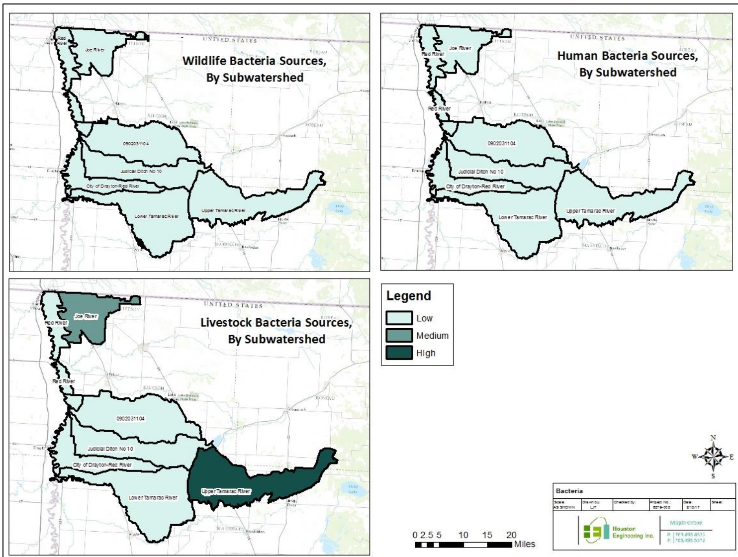
Figure 8: Ranked HUC-10 subwatersheds based upon magnitude of bacterial delivery to the outlet of the LRRW. Note: Boundaries used within bacteria risk assessment and PTMApp are different, as they rely upon existing hydroconditioned digital elevation models.
