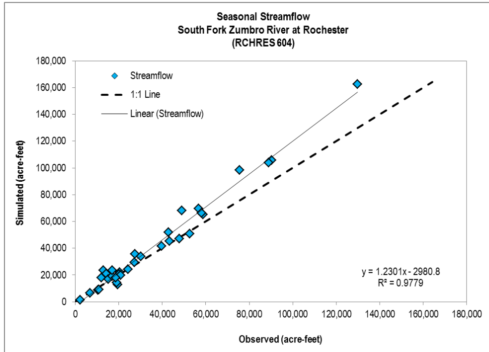
Figure 4-26. Seasonal Streamflow 1:1 Plot for South Fork Zumbro River at Rochester (RCHRES 604) for Model Validation (1996-2003).
