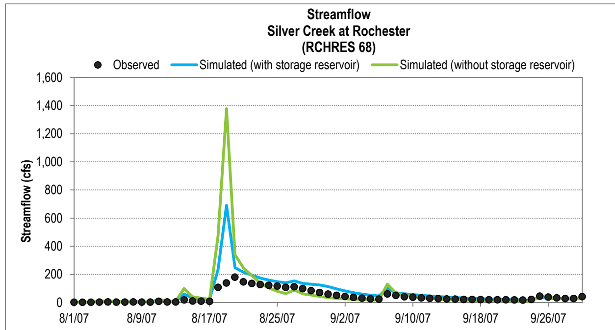
Figure 4-6. Observed and Simulated streamflow at the Silver Creek station.
