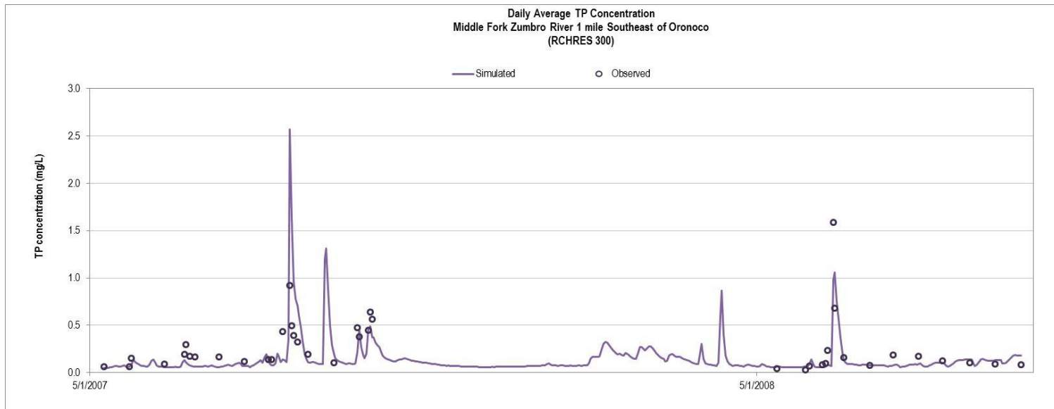
Figure D-4. Daily Average Total Phosphorus Concentrations for Middle Fork Zumbro River 1 mile Southeast of Oronoco (RCHRES 300)
