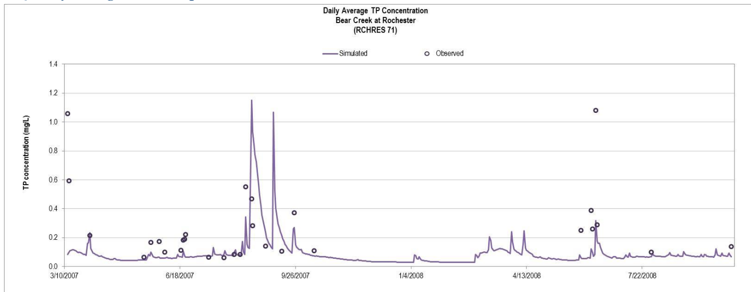
Figure D-5. Daily Average Total Phosphorus Concentrations for Bear Creek at Rochester (RCHRES 71)
