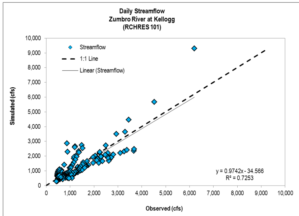
Figure A-44. Daily Streamflow 1:1 Plot for Zumbro River at Kellogg (RCHRES 101)
