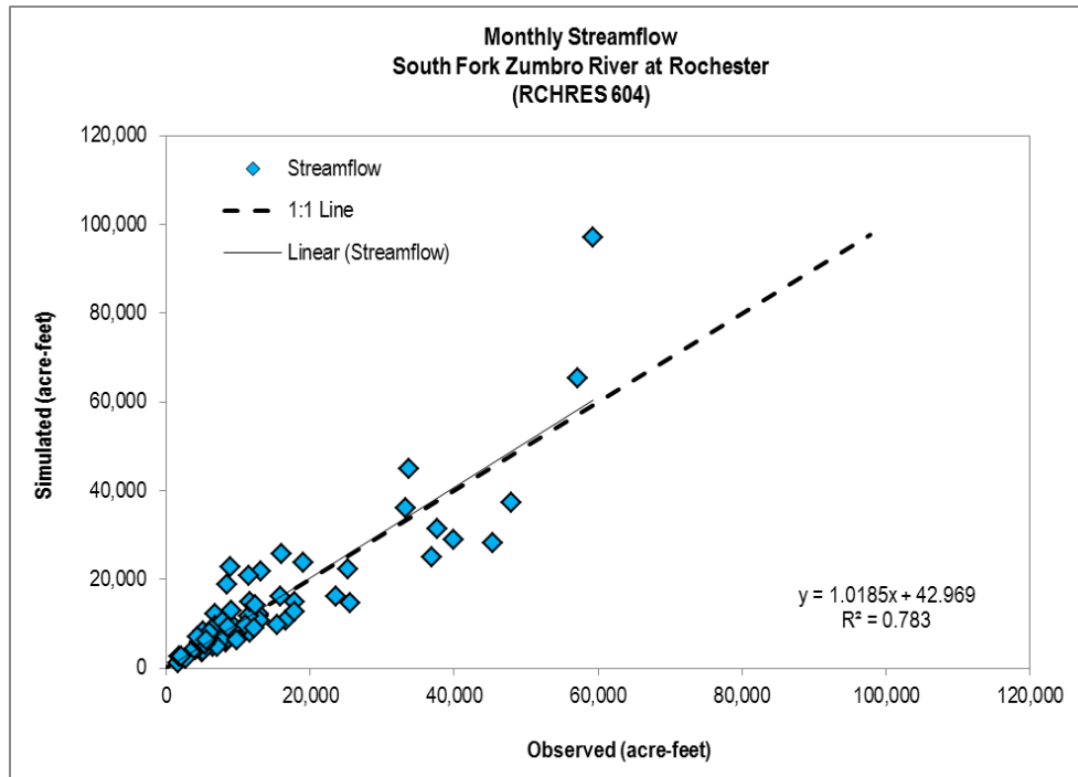
Figure 4-9. Monthly Streamflow 1:1 Plot for South Fork Zumbro River at Rochester (RCHRES 604) for Model Calibration (2004-2009).
