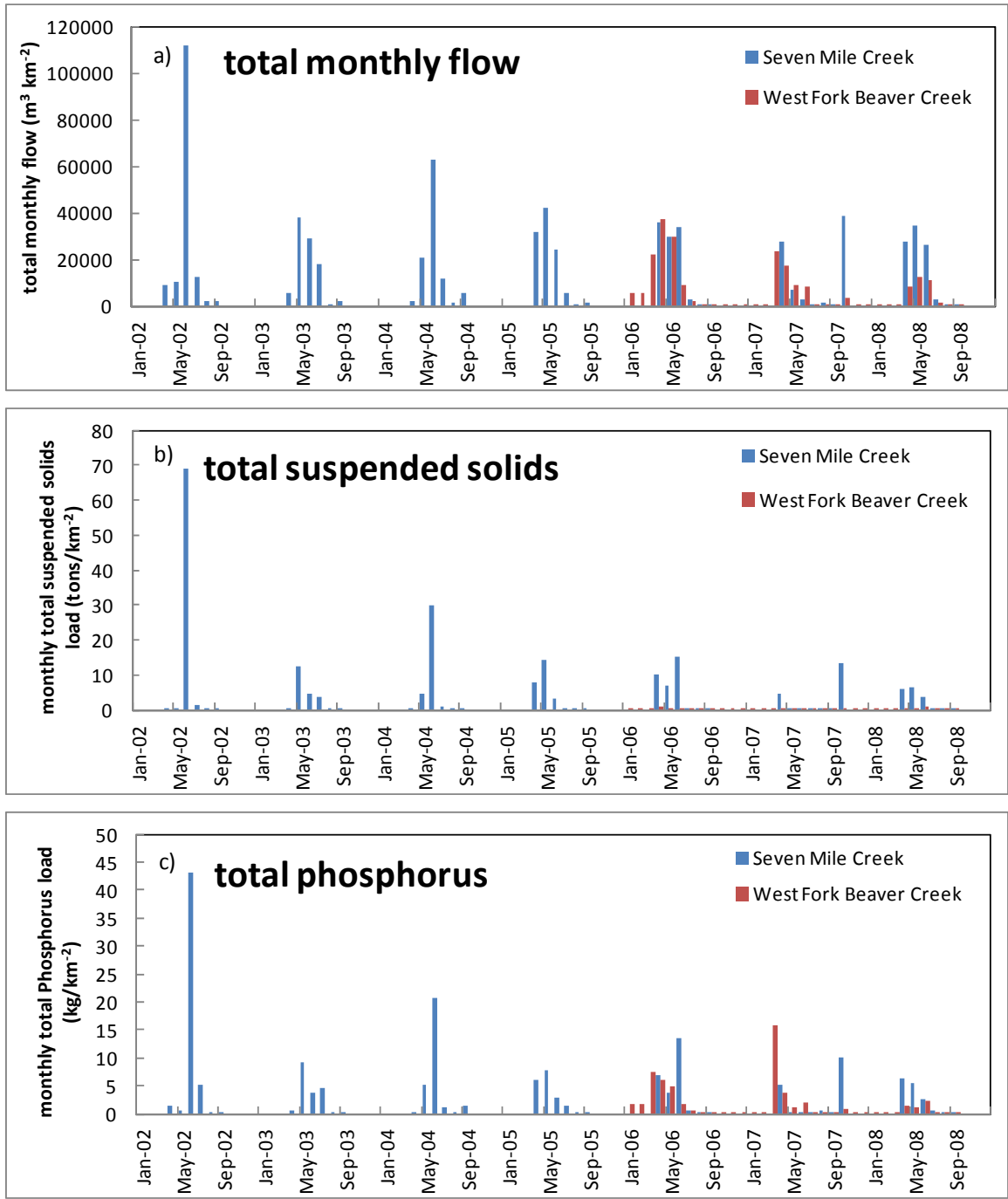
Figure 7. Bar graphs showing area-normalized a) water, b) sediment, and c) phosphorus loads at the watershed outlet under baseline conditions for the two study watersheds. Data shown reflect the period of monitoring data available for each watershed. Tabular data are contained in Appendix A.
