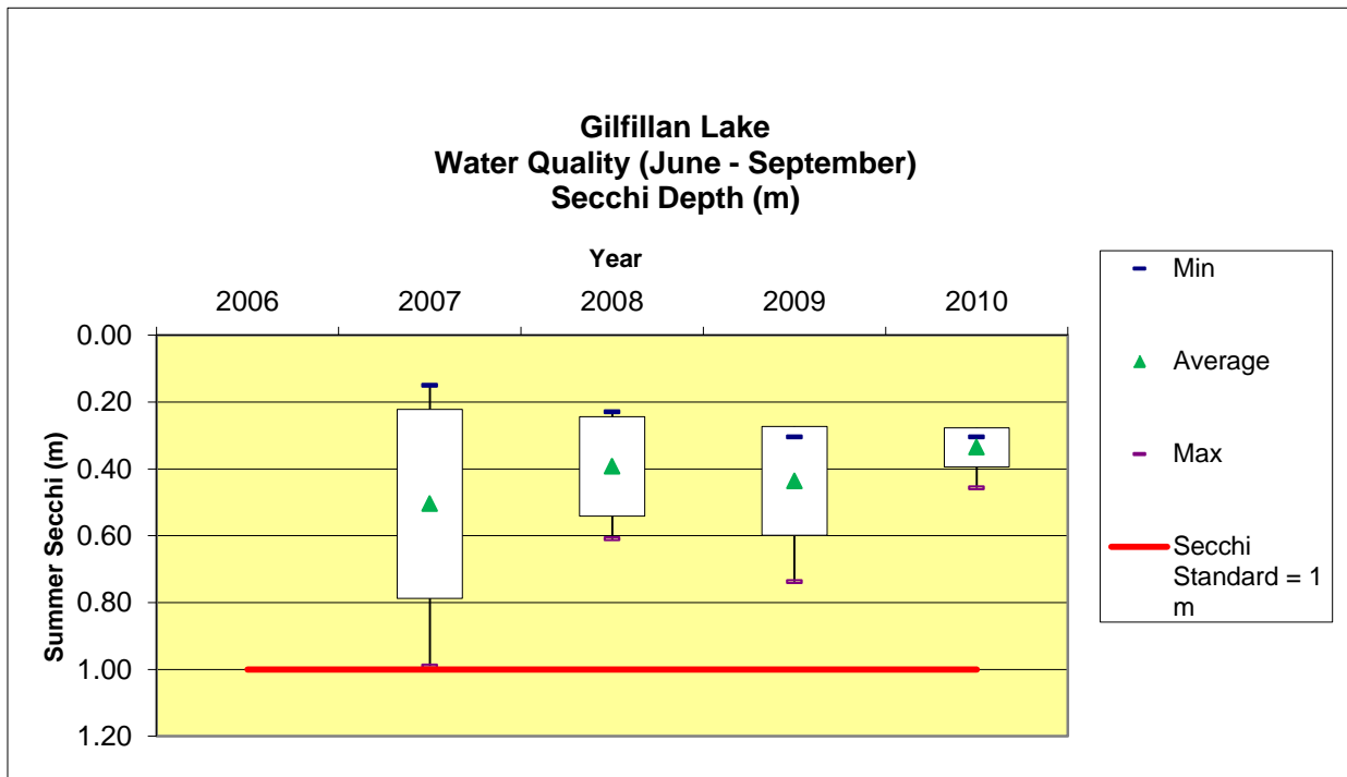
Figure 3.15. Gilfillan Lake Secchi Depths (June – September).
