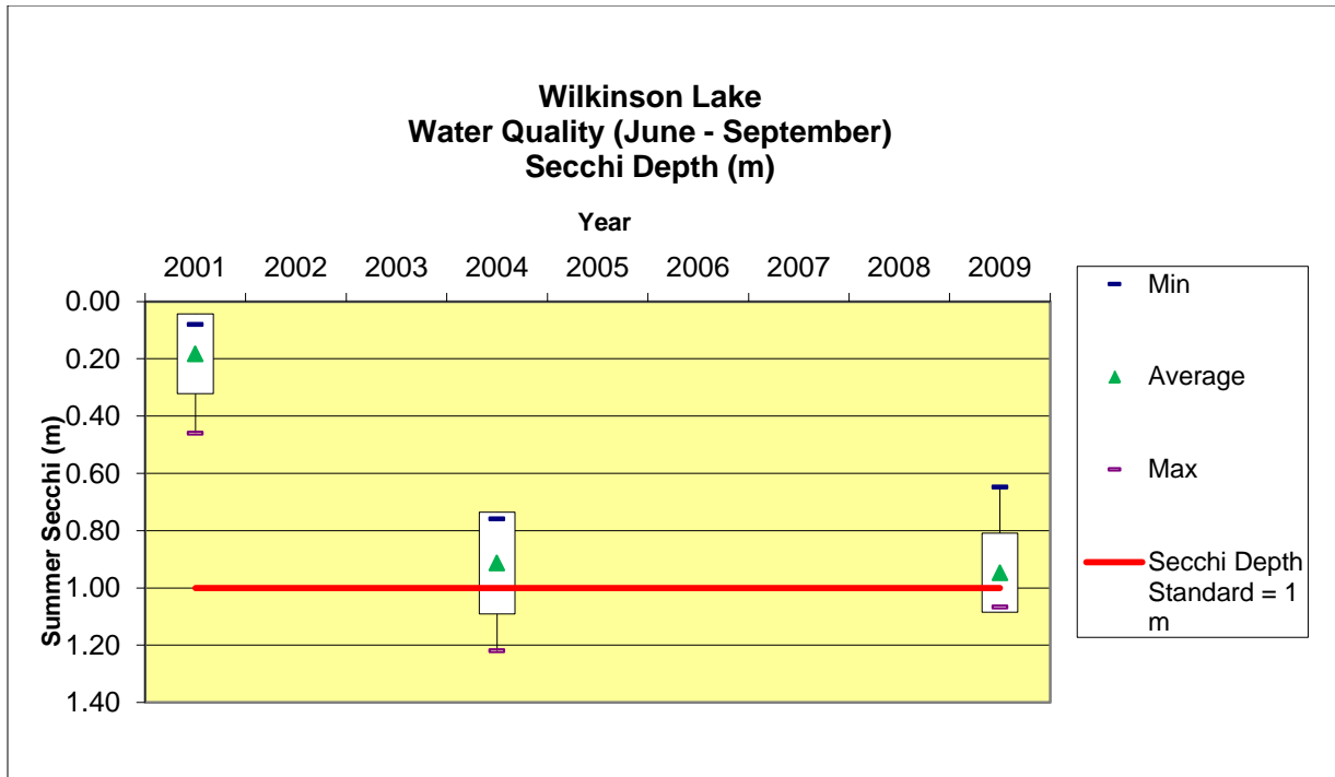
Figure 3.18. Wilkinson Lake Secchi Depths (June – September).
