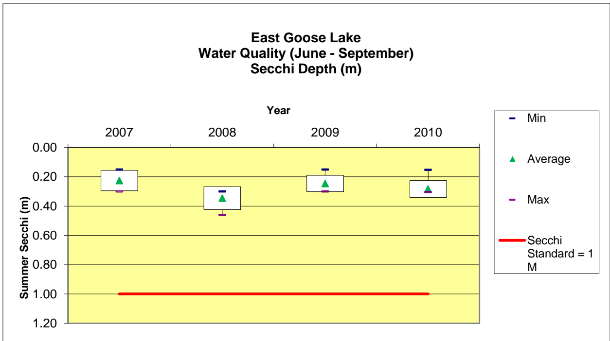
Figure 3.9. East Goose Lake Secchi Depths (June – September).
