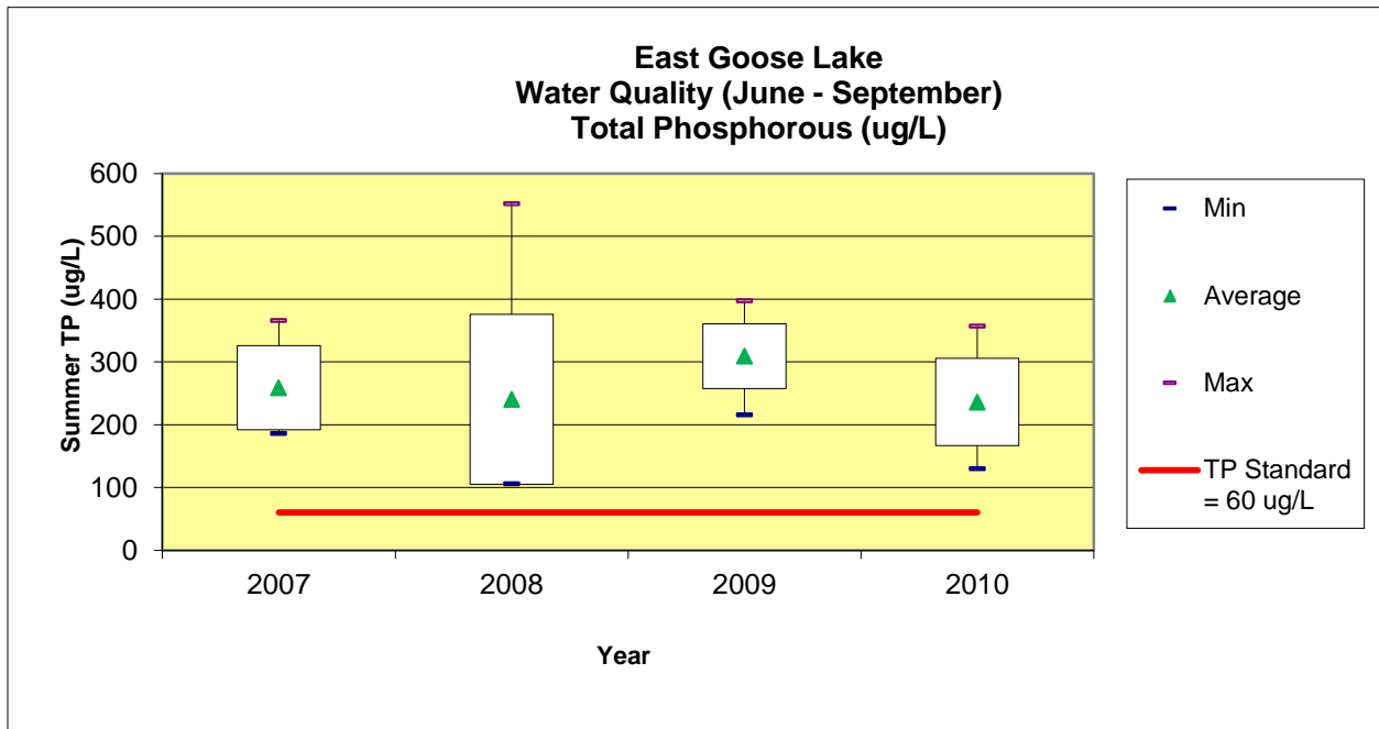
Figure 3.7. East Goose Lake Total Phosphorus Concentrations (June – September).
