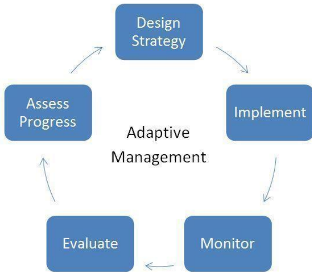
Figure 3.1. Adaptive management.
