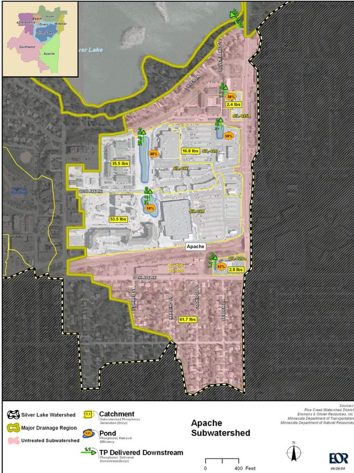
Figure 17. Apache Subwatershed
