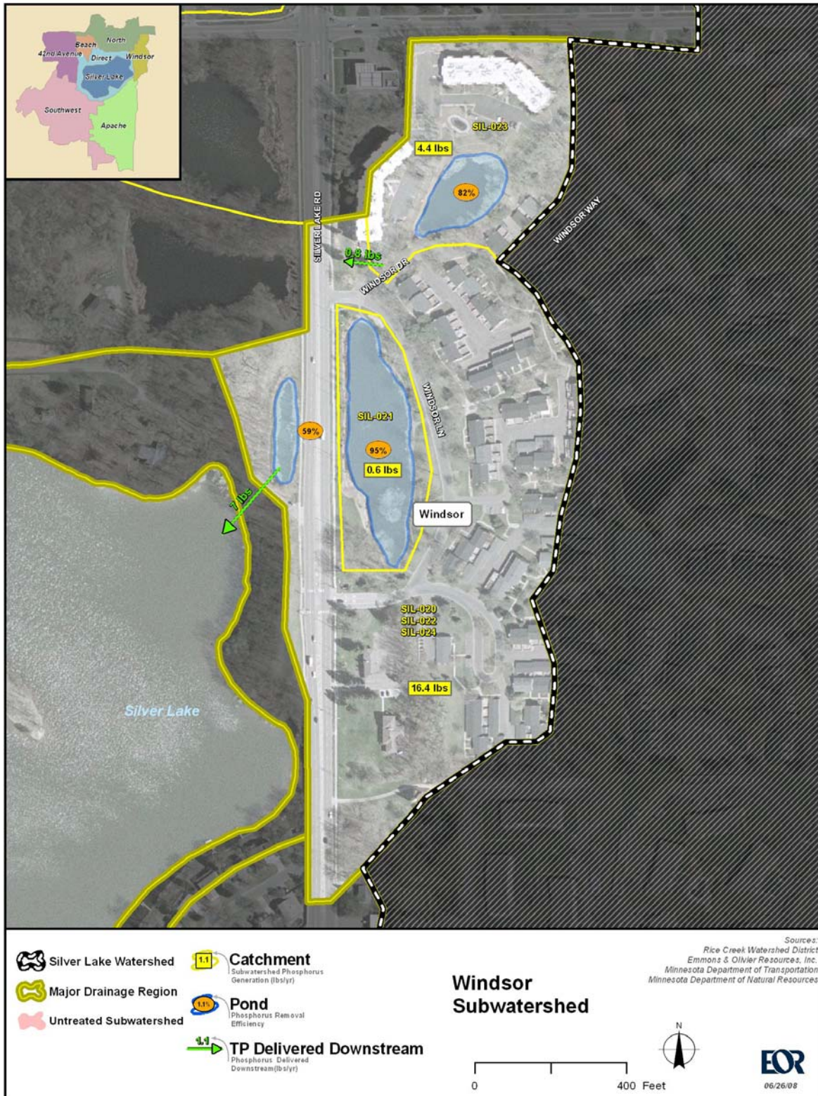
Figure 21. Windsor Subwatershed
