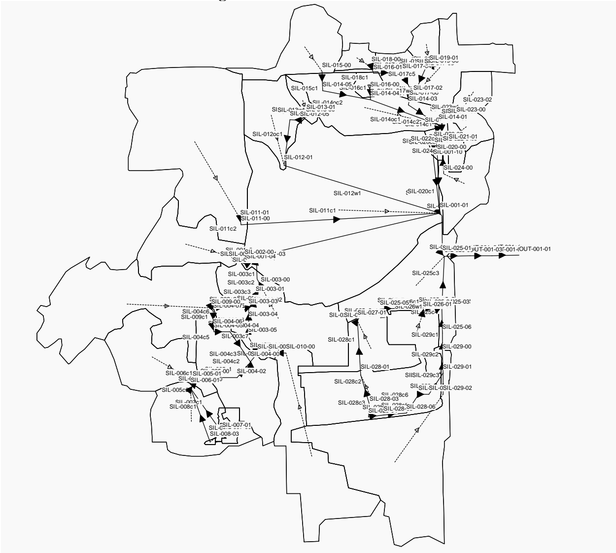
Figure A-3: StormNET Model.
