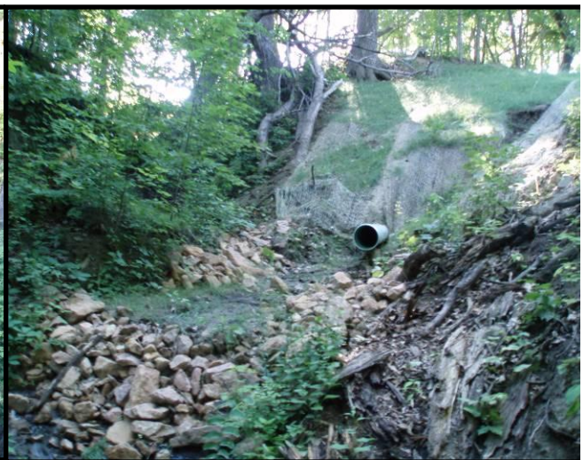
Figure 4.31 New pipe outlet from golf course (Site 15)
