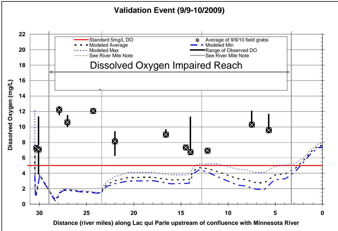
Figure 6.1 Lac qui Parle River validation event dissolved oxygen longitudinal profile (20090909_LqP_015.xls).
