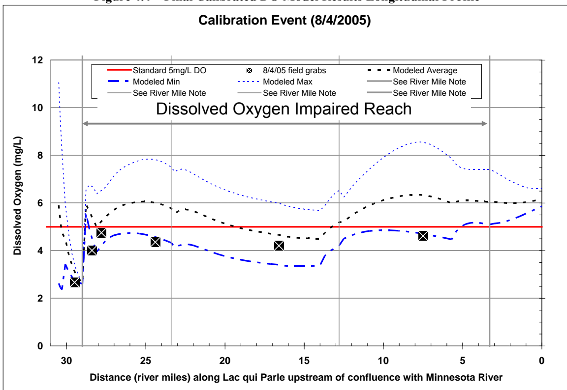
Figure 4.4 – Final Calibrated DO Model Results Longitudinal Profile
