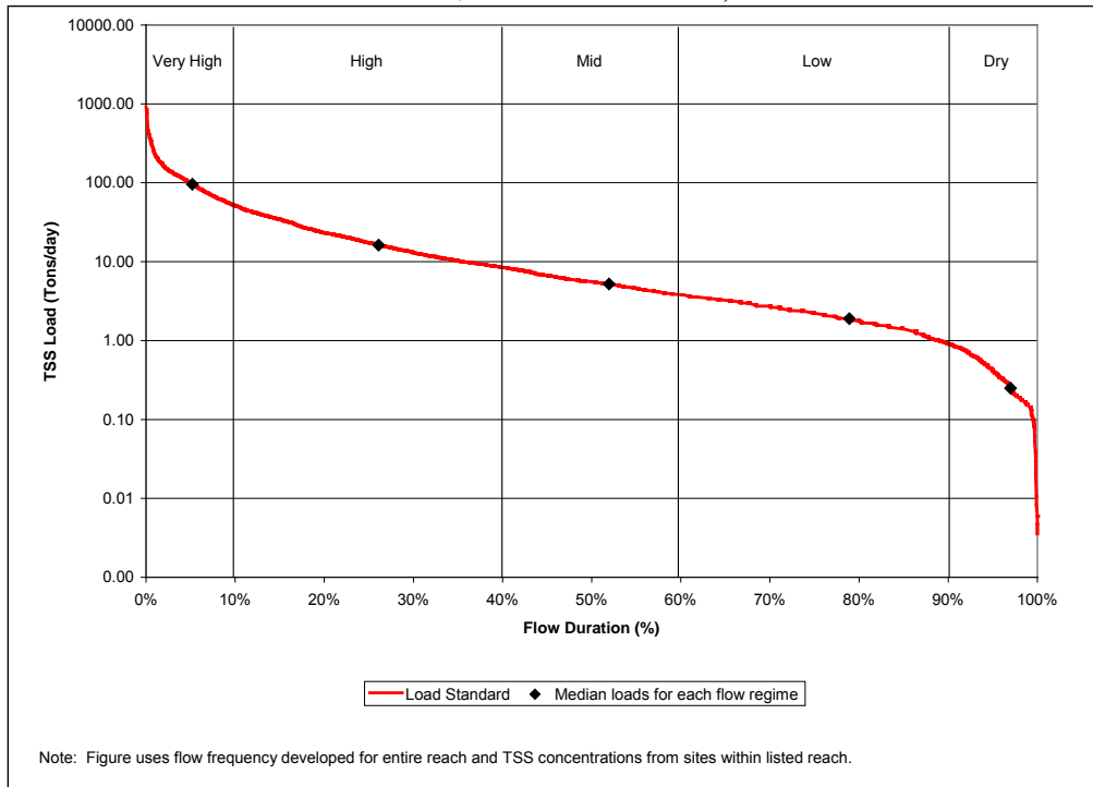
Figure 3.4 – TSS Load Duration Curve for Lac qui Parle River (West Br. Lac qui Parle River to Ten Mile Creek, AUID 07020003-501)
