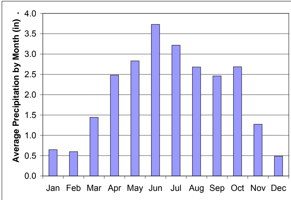
Figure 1.4 – Average Monthly Distribution of Precipitation at Madison, MN.
