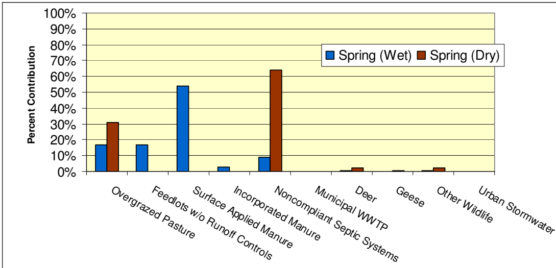
Figure A.9: Estimated Relative Delivered Bacteria Load by Source, Season, and Moisture Condition in the Watershed Draining to North Fork Yellow Bank River (AUID 07020001-510, South Dakota Border to Yellow Bank River mainstem)
