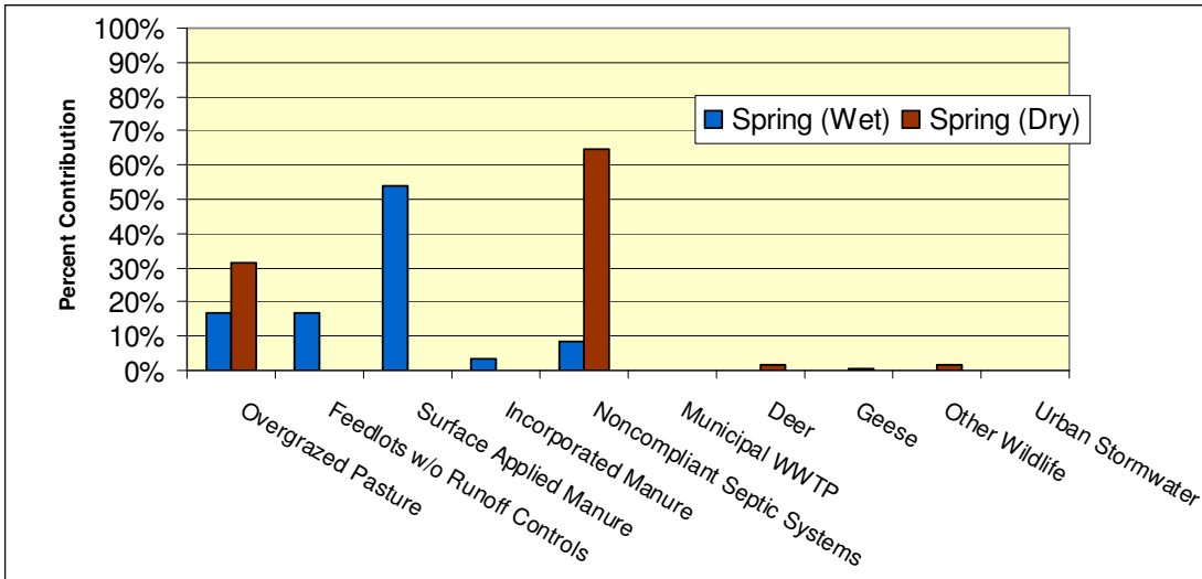
Figure A.11: Estimated Relative Delivered Bacteria Load by Source, Season, and Moisture Condition in the Watershed Draining to Yellow Bank River (AUID 07020001-525, North Fork Yellow Bank River to Minnesota River)
