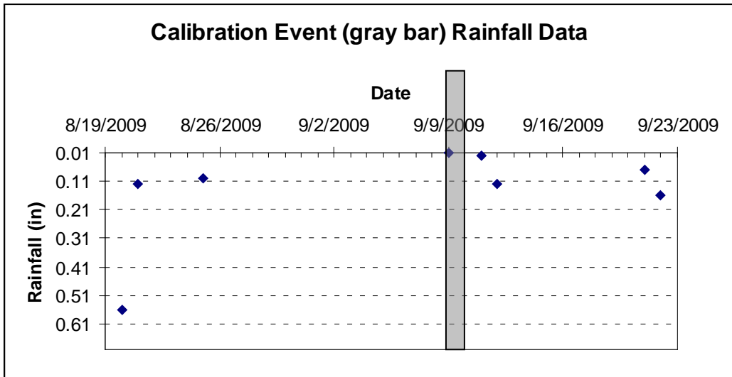
Figure 3.2 Rainfall recorded around the 9/9-10/2009 event.
