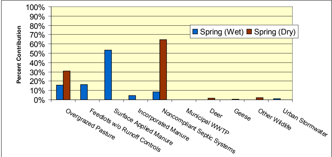
Figure 2.14 – Estimated Delivery Potential by Season, Flow Condition, and Source for Lac qui Parle River – W. Branch to Ten Mile Creek (AUID 07020003-501)
