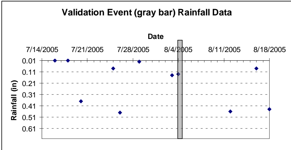
Figure 3.1 Rainfall recorded around the 8/4/2005 event.
