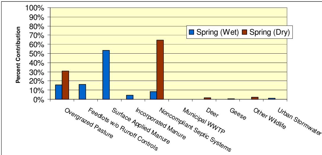
Figure A.7: Estimated Relative Delivered Bacteria Load by Source, Season, and Moisture Condition in the Watershed Draining to Lac qui Parle River (AUID 07020003-501, W. Branch Lac qui Parle River to Ten Mile Creek)
