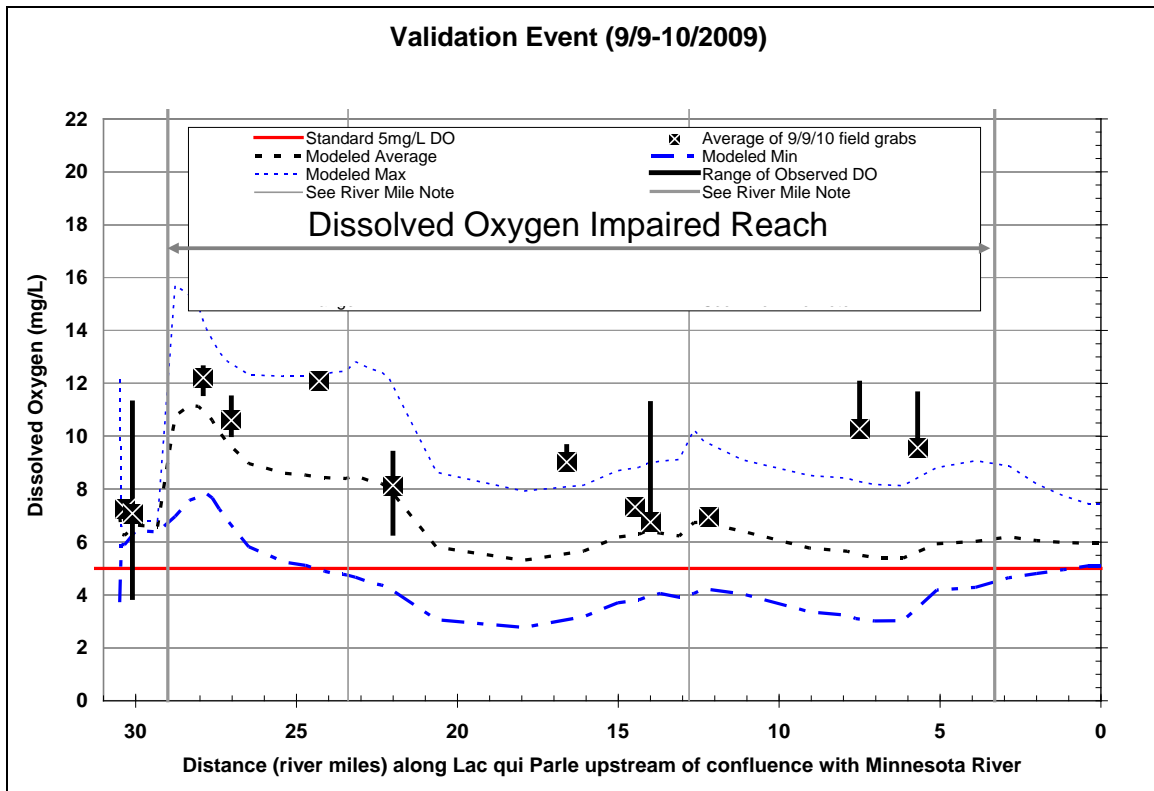
Figure 6.2 Lac qui Parle River validation event dissolved oxygen longitudinal profile (20090909_LqP_019.xls).
