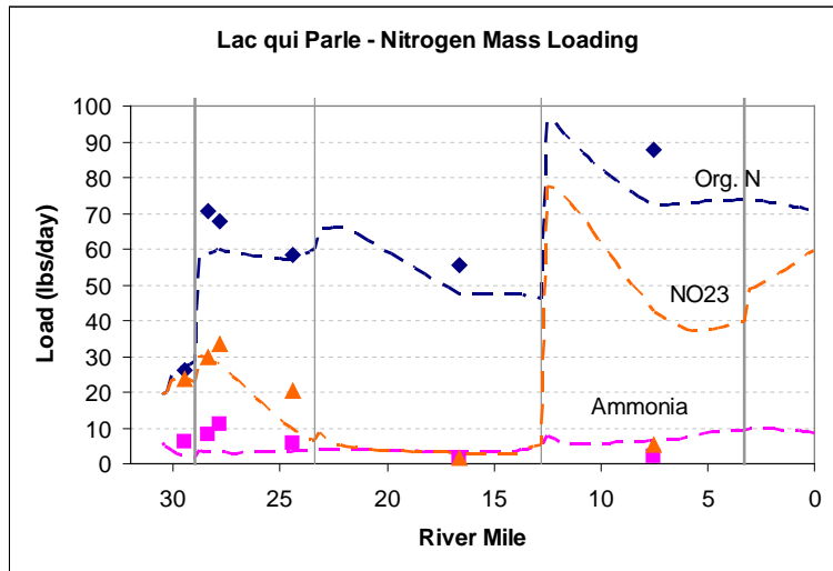
Figure 5.5 Final calibration mass load plot of nitrogen parameters.
