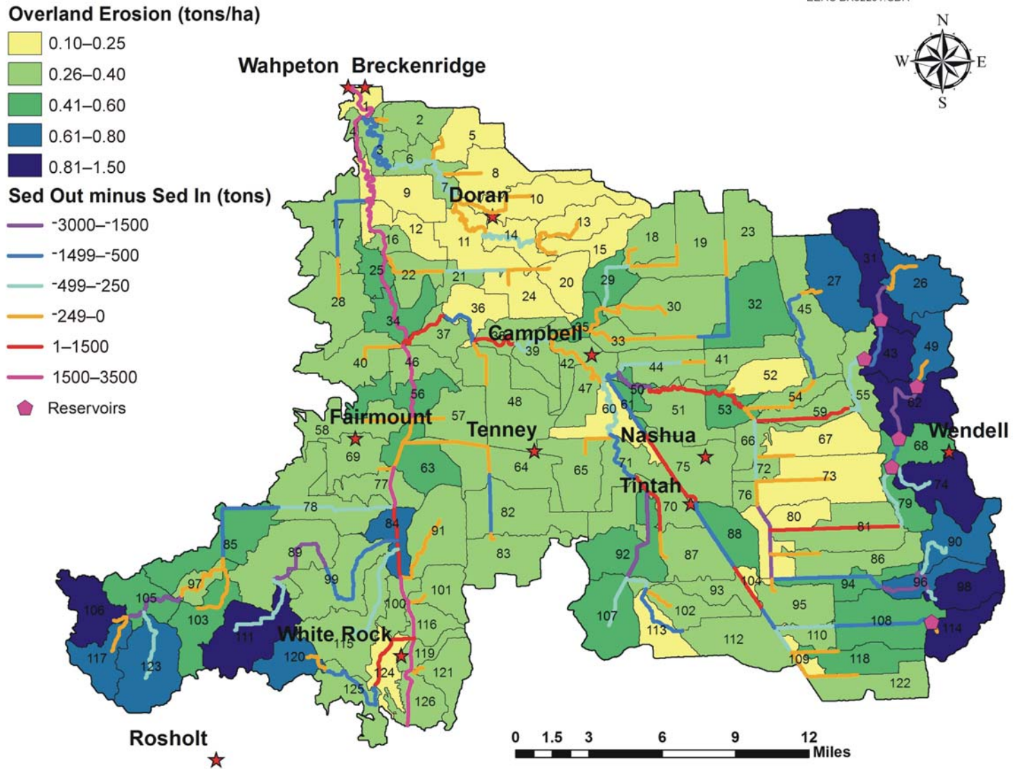
Figure 29. Estimated average annual sediment erosion from the landscape and net sediment loading (upstream inputs minus subbasin outputs) within the waterways of the Bois de Sioux River Watershed.
