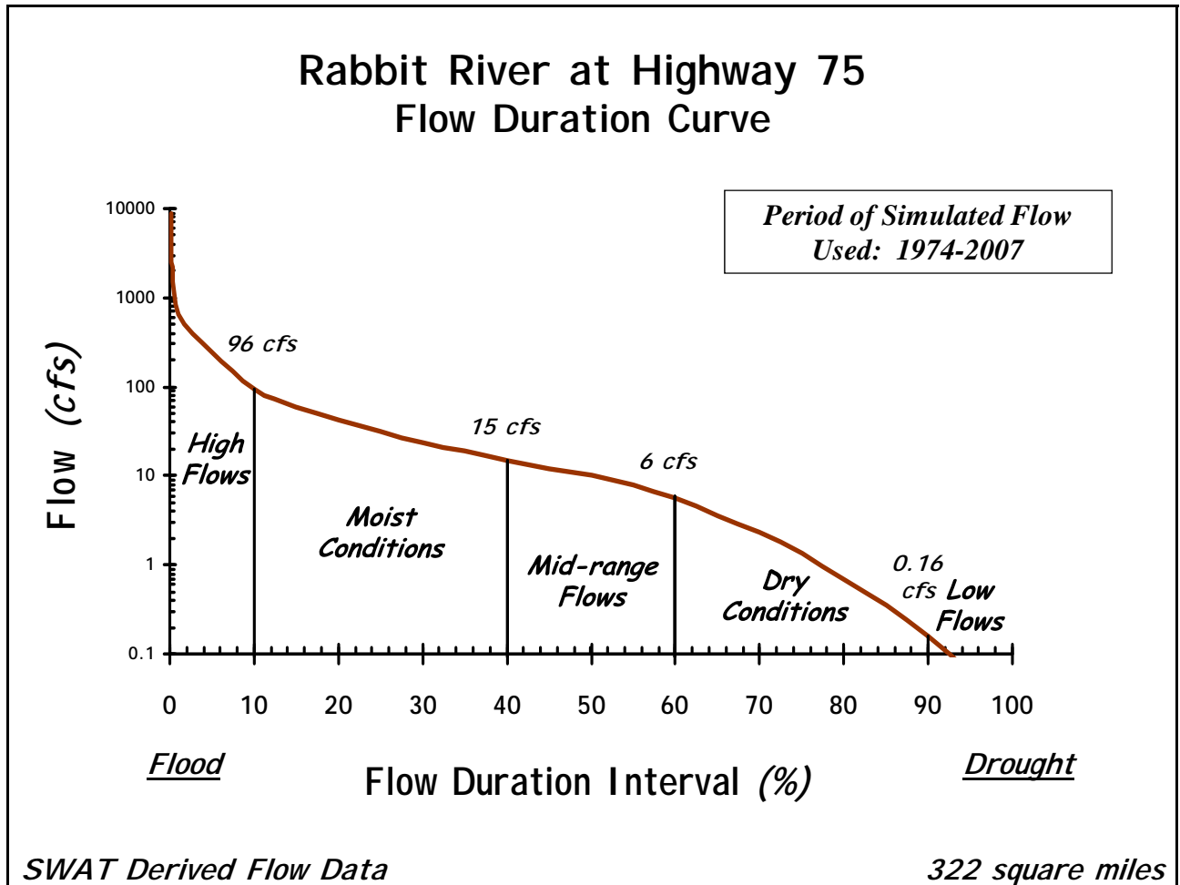
Figure 5 – Flow Duration Curve
