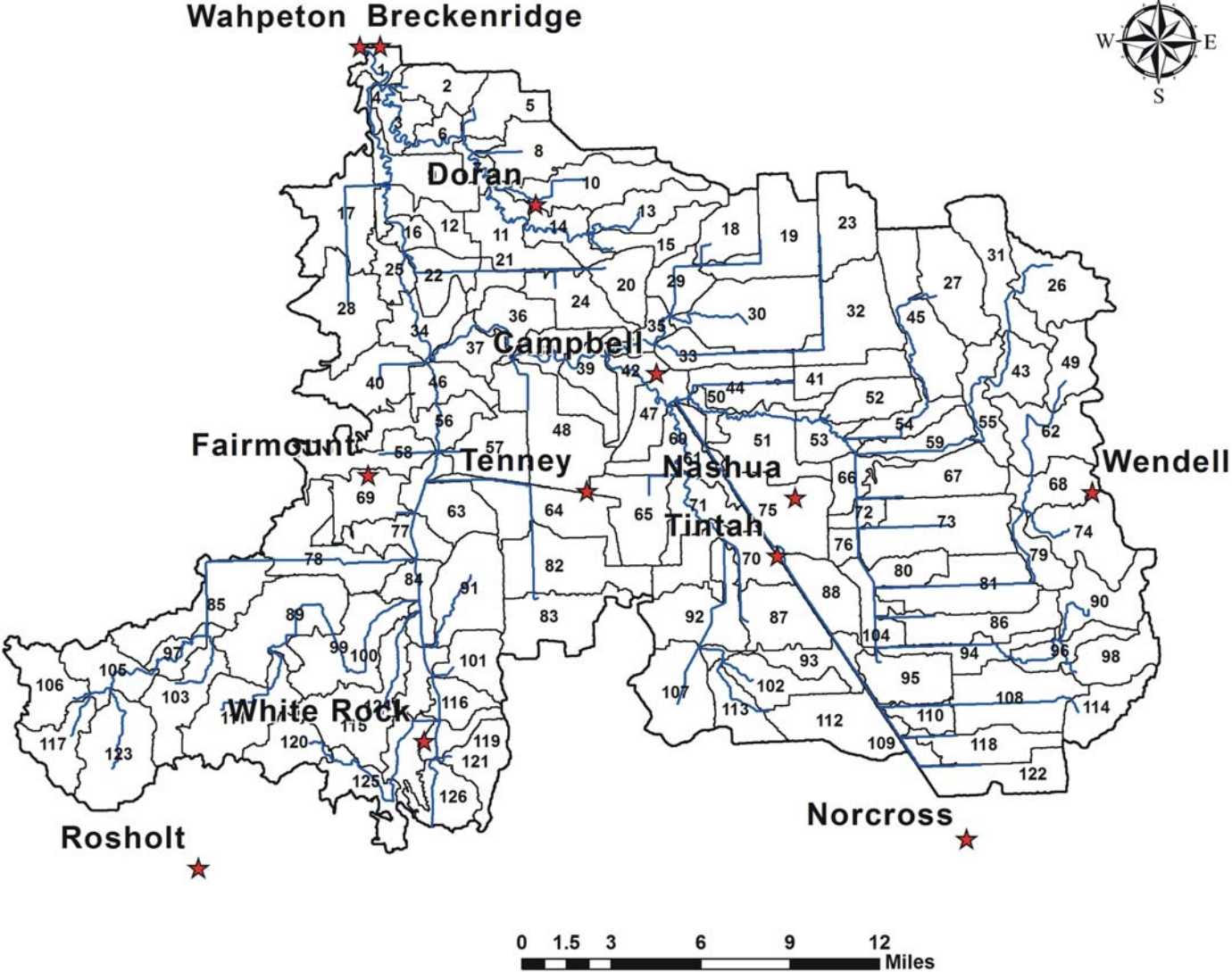
Figure 5. Location of the subbasins defined within the Bois de Sioux Watershed.
