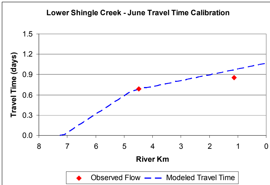
Figure 3.12. Time of travel calibration plot, June travel time calibration
