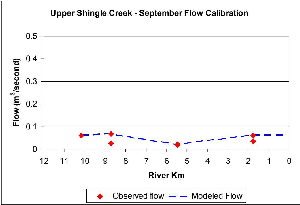
Figure 3.11. Final flow calibration plot for Upper Shingle Creek with diffuse source inflows, September flow calibration.
