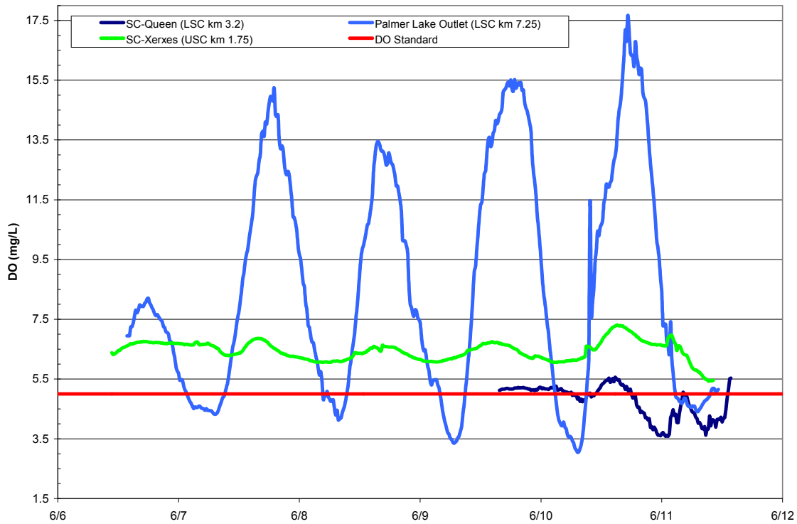
Figure 2.32. June 2008 survey continuous dissolved oxygen concentrations.
