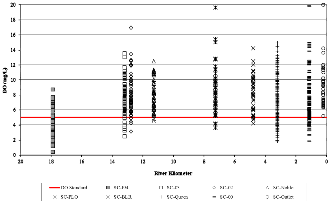
Figure 1.2. Dissolved oxygen data for all Shingle Creek stations by river kilometer.
