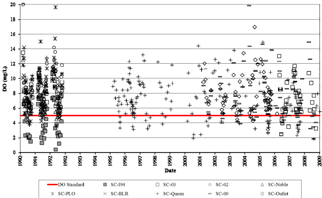
Figure 1.1. Dissolved oxygen data for all Shingle Creek stations by year.
