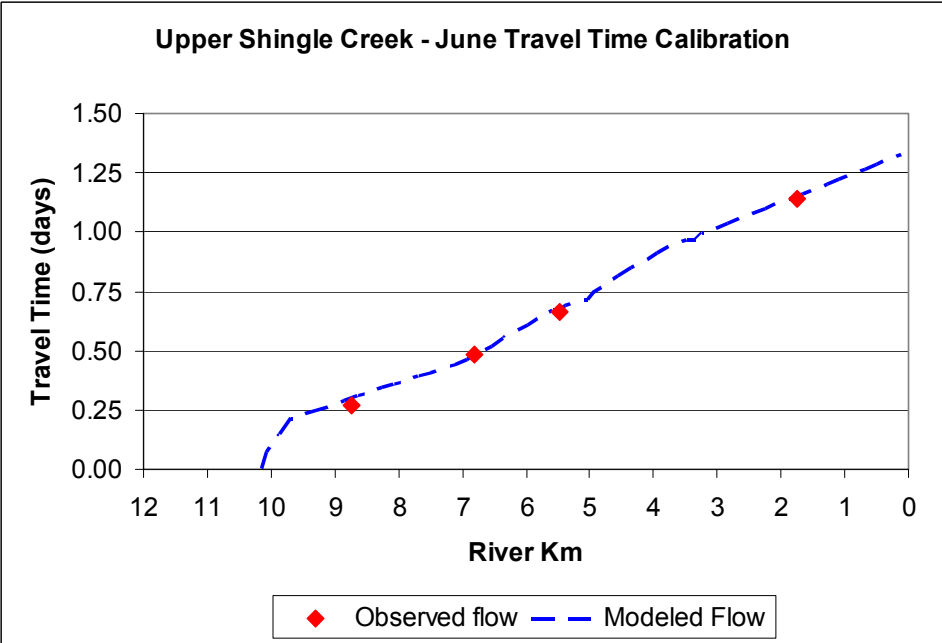
Figure 3.14. Time of travel calibration plot, June travel time calibration.
