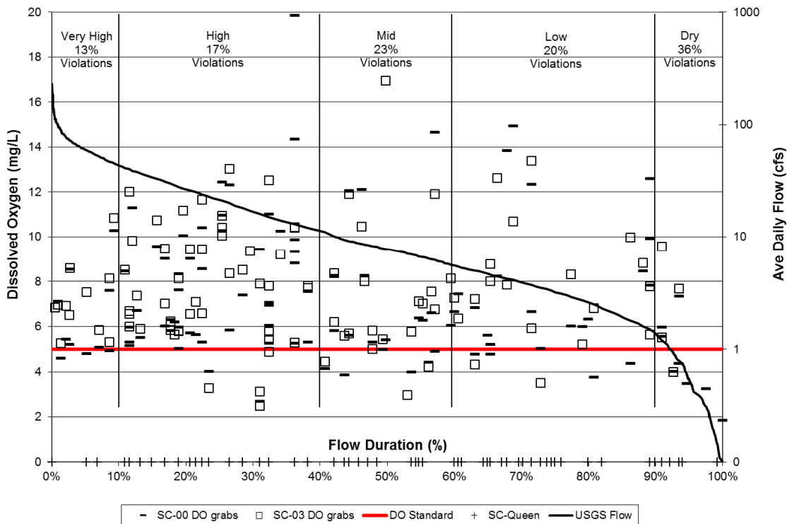
Figure 1.6. Dissolved oxygen flow duration plot using average daily flow data from the USGS (SC-Queen) station.
