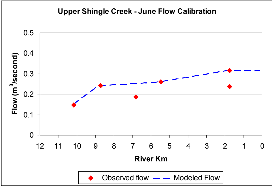
Figure 3.10. Final flow calibration plot for Upper Shingle Creek with diffuse source inflows, June flow calibration.
