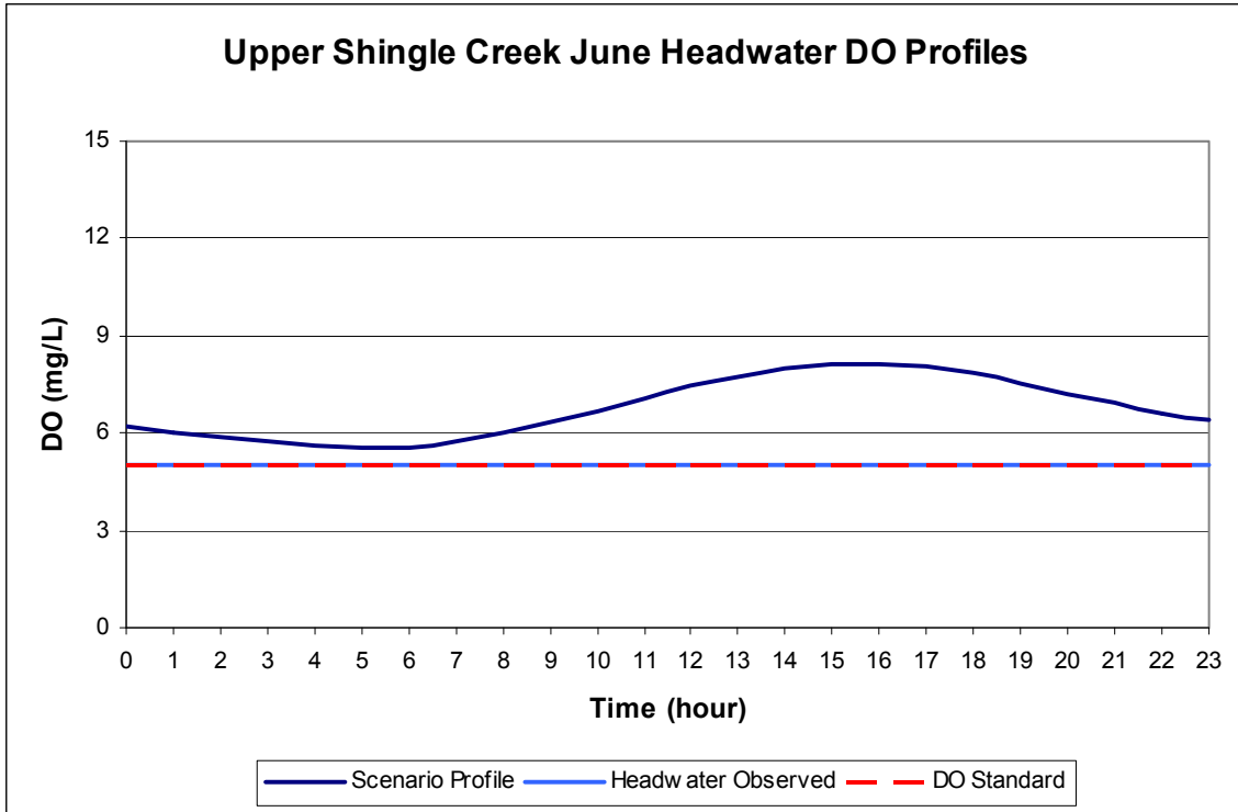
Figure 3.1. Higher flow scenario 1 DO headwater profile.
