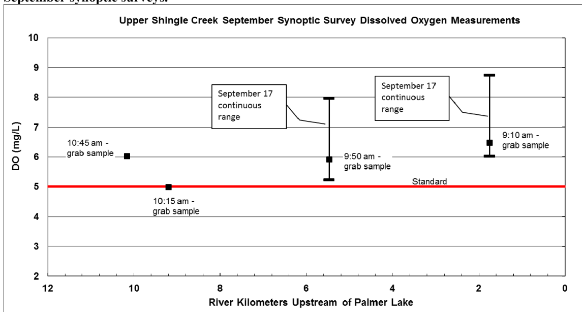
Figure 2.36. Upper Shingle Creek dissolved oxygen field grabs and continuous data collected during the September synoptic surveys.
