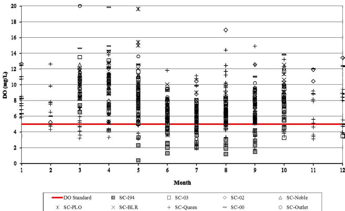
Figure 1.3. Dissolved oxygen data for all Shingle Creek stations by month, regardless of year.
