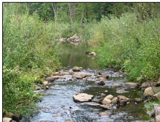
(Left) Seven rock vanes were placed in Pike Creek between Hemlock Lane and Pike Lake in Maple Grove.
