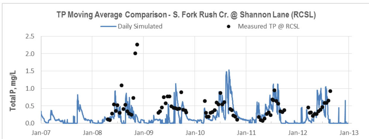
Figure 25. Simulated and observed TP concentrations at station RCSL (S. Fork Rush Creek @ Shannon Lane). Simulated values are plotted as five day moving averages.
