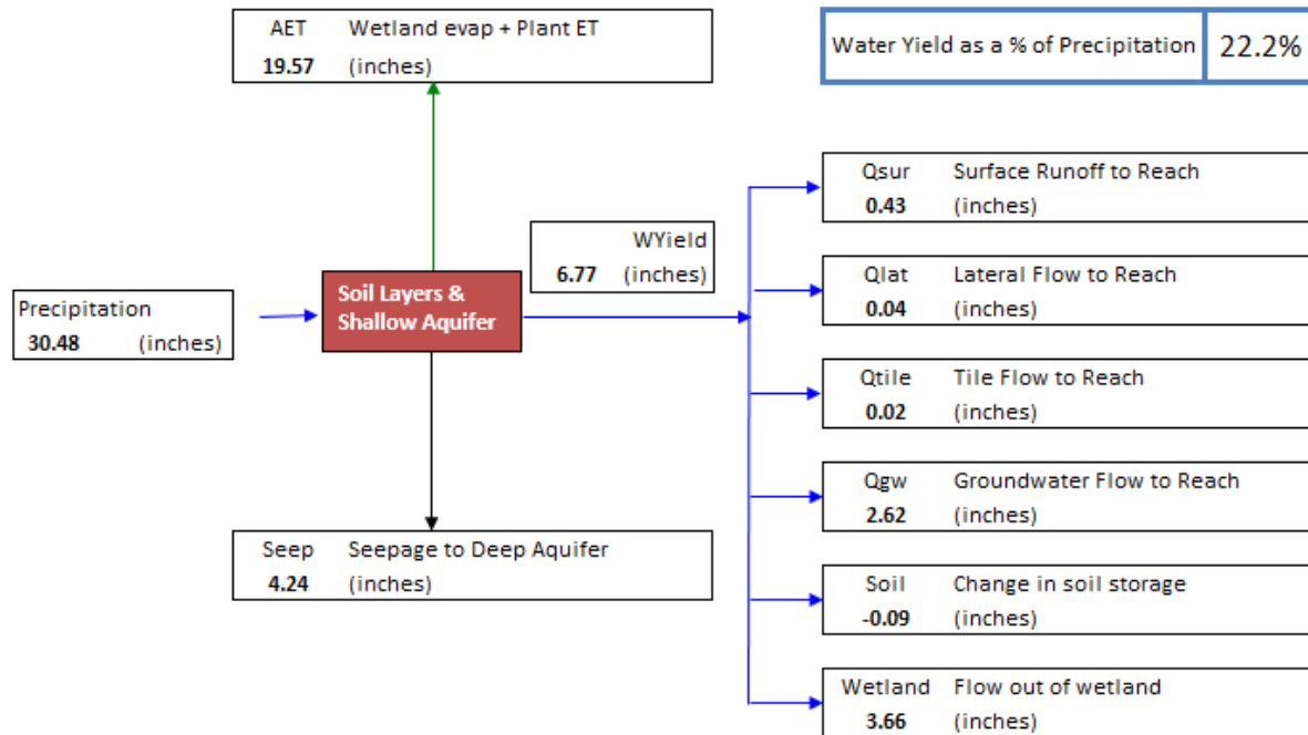
Figure 3. Elm Creek watershed SWAT model simulated annual average water balance (2000-2012) 2
