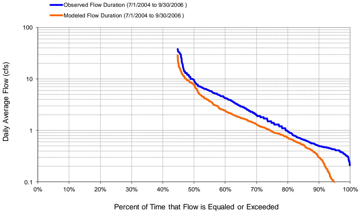
Figure 142. Flow exceedence at Knife River at Nappa Road
