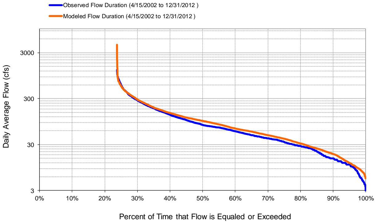
Figure 184. Flow exceedence at Poplar River near Lutsen
