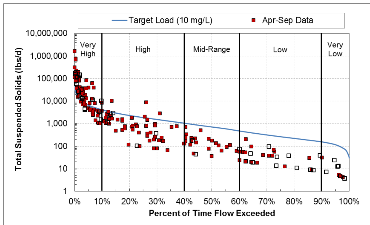
Figure 24. TSS load duration curve, Big Sucker Creek (Sucker River; 04010102-555). Hollow points indicate samples during months when the standard does not apply.
