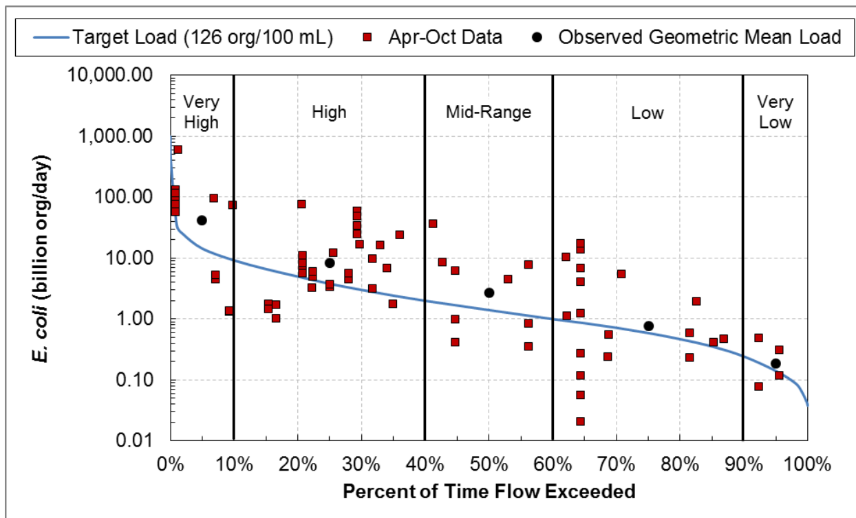
Figure 29. E. coli load duration curve, Skunk Creek (04010102-528).
