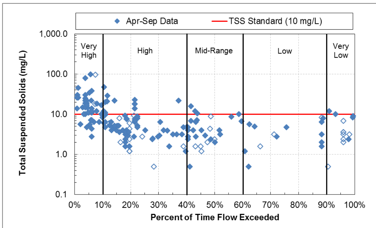
Figure 7. TSS water quality duration plot, Beaver River. (AUID 04010102-501), 2007–2011, 2013–2016. Hollow points indicate samples during months when the standard does not apply.
