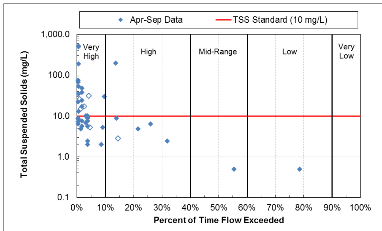
Figure 10. TSS water quality duration plot, Talmadge River.
