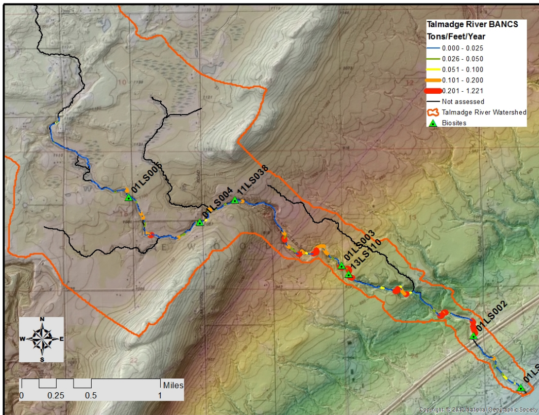
Figure 22. Talmadge River BANCS predicted erosion rates (MPCA 2017).
