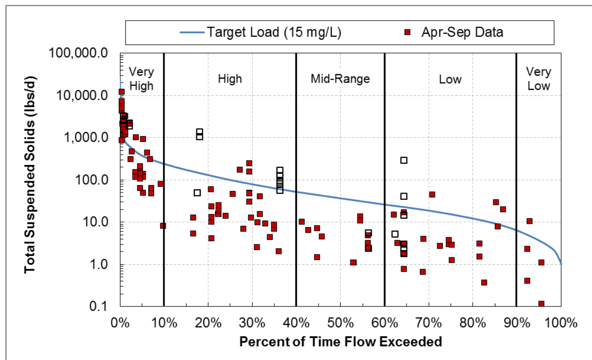
Figure 28. TSS load duration curve, Skunk Creek (04010102-528).
