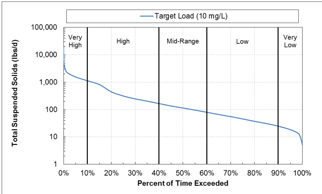
Figure 27. TSS load duration curve, Little Knife River (East Branch Little Knife River; 04010102-840). No data are available during the TMDL period (2007-2016); older data are provided in Section 3.3.5.
