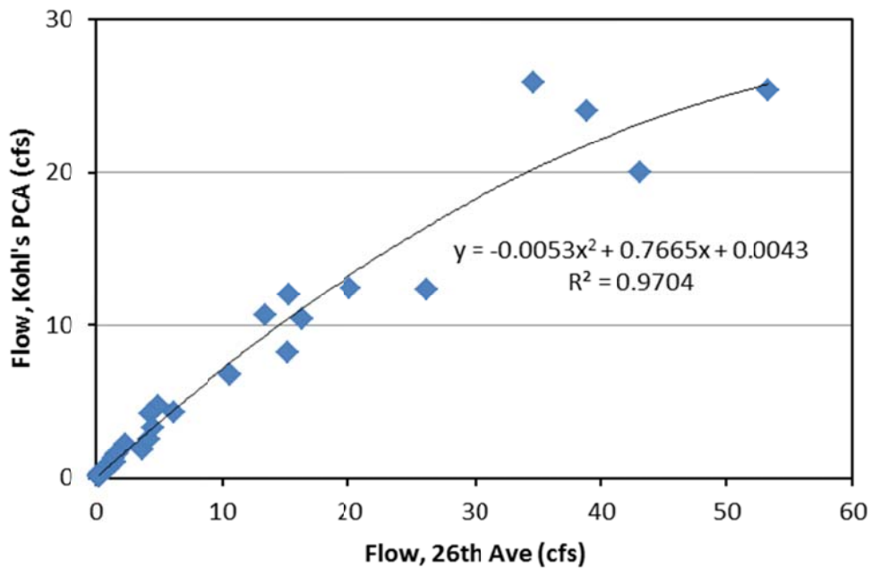
Figure 8. Regression equation to predict flow at the Kohl's MPCA site based on observed flow at the 26 th Ave site, based on SWMM simulated stream flow in 2008.
