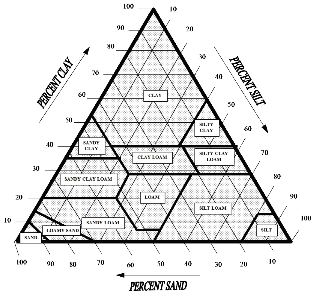
Figure 1 USDA Soil Textural Triangle
