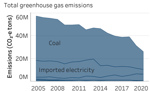
Trends in greenhouse gas emission sources
