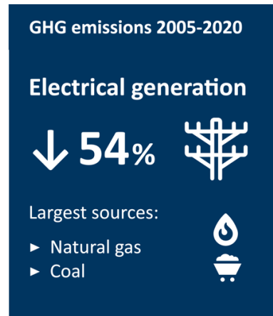
Electricity generation sector: 2005 to 2020
