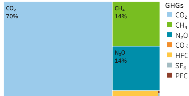
Net 2020 GHG emissions in Minnesota by gas, in CO 2 -equivalent tons (includes carbon storage)
