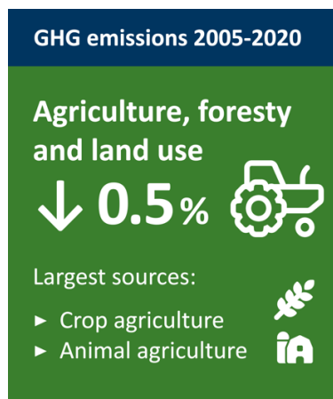
Agriculture, Forestry & Land use sector: 2005 to 2020
