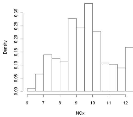
Histogram of NOx
