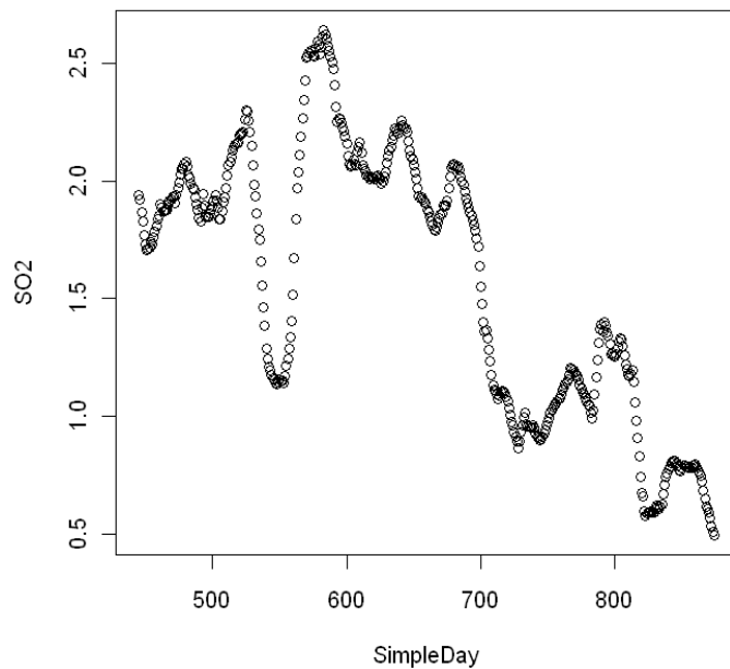
SO 2 Emissions Over Time (tpd)
