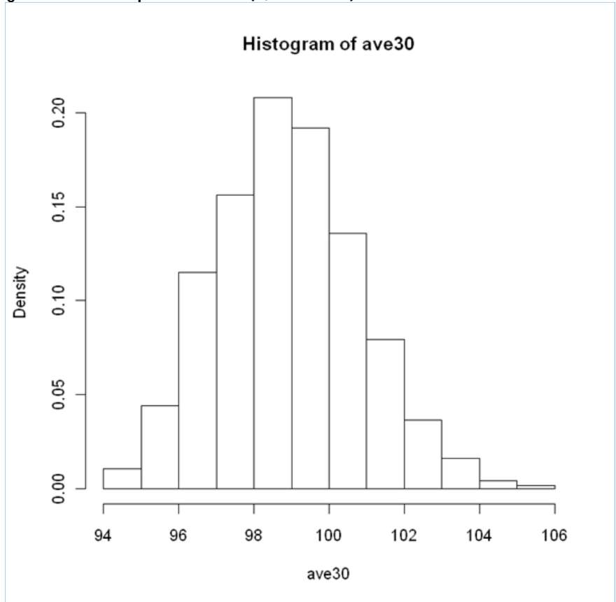
Histogram of Bootstrap Distribution (R, se = 1.896)
