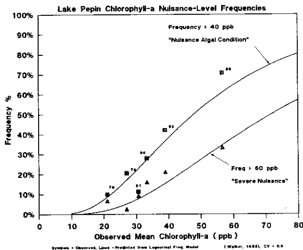
Figure 8.—Chlorophyll a Nuisance Level Frequencies for Lake Pepin. Log-normal frequency distributions (Walker, 1985a) have been used to predict frequency of algal blooms as a function of summer-mean chl a . Based on six summers of data, observed chlorophyll a interval frequencies for Lake Pepin agree with frequencies predicted from the log normal distribution model.
