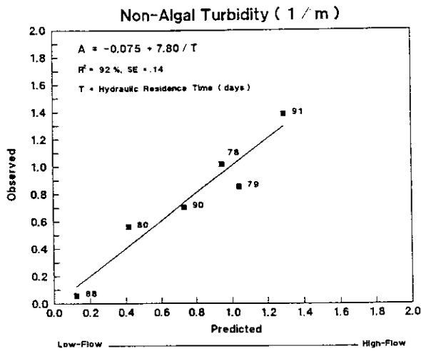
Figure 5.—Summer-mean non-algal turbidity measures for Lake Pepin. For Lake Pepin, non-algal turbidity (calculated as per Table 2) is highly correlated with hydraulic residence time ( r^2=0.92 ) and may be predicted based on hydraulic residence time.
