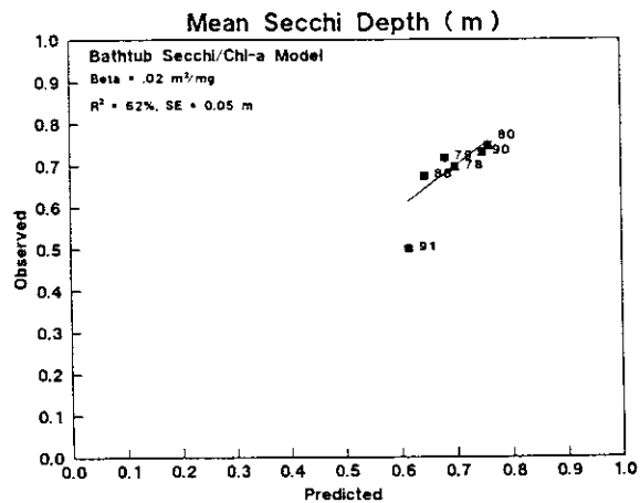
Figure 7.—Observed vs. Predicted Secchi transparency for Lake Pepin. Secchi transparency is predicted based on chlorophyll a and non-algal turbidity.
